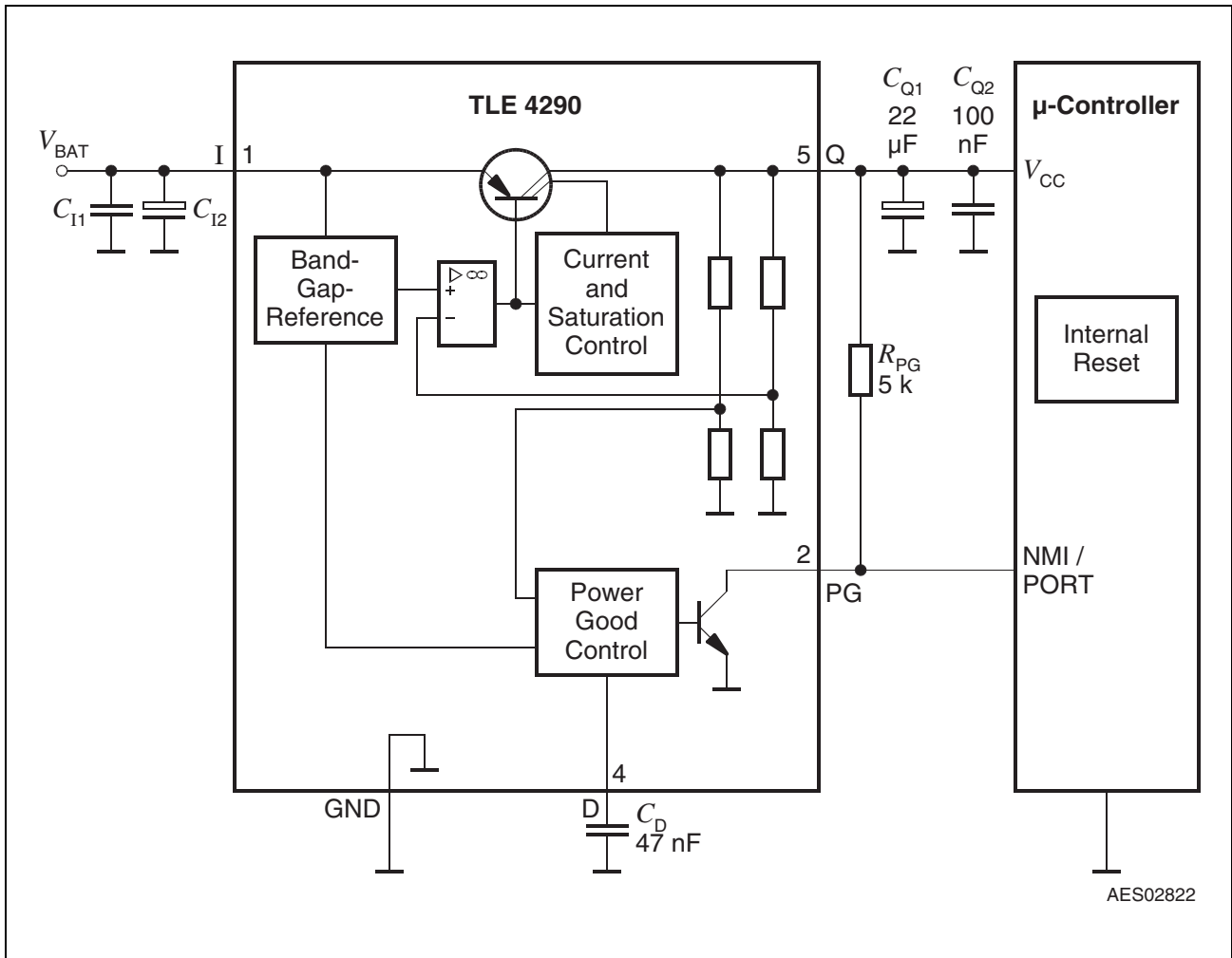
Figure 4 Application Diagram
