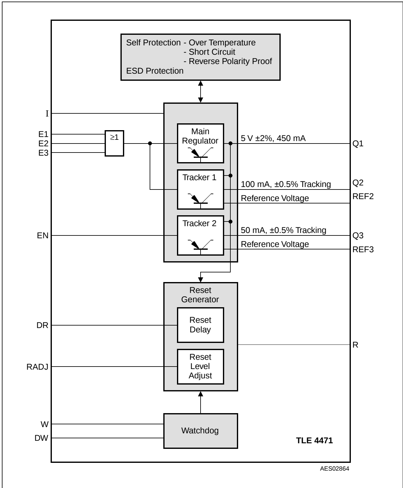
Figure 1 Block Diagram
