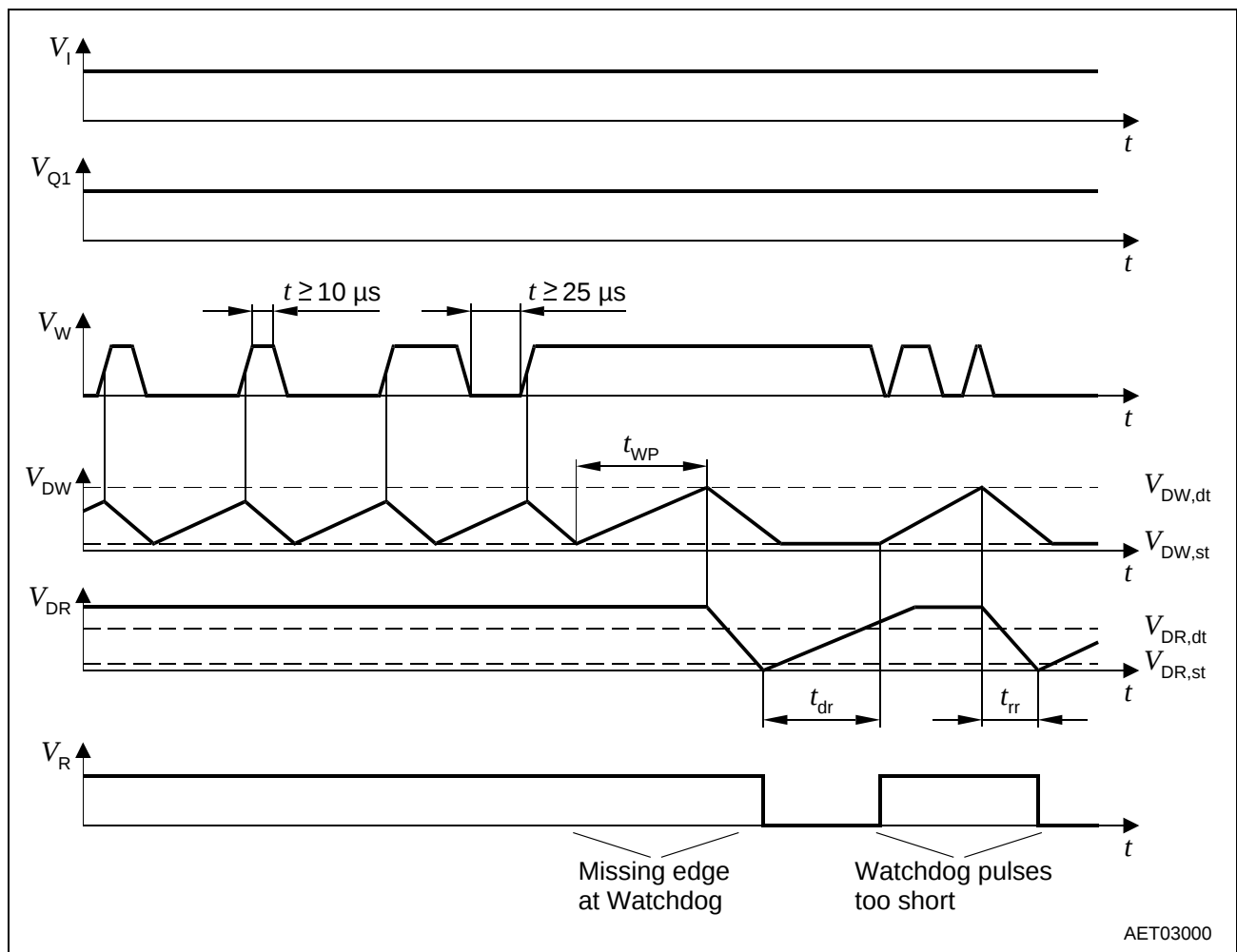
Figure 7 Watchdog Timing
