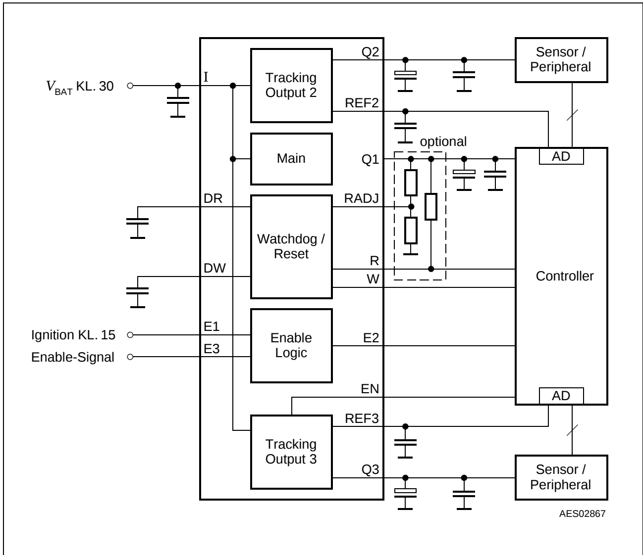
Figure 4 Application Diagram
