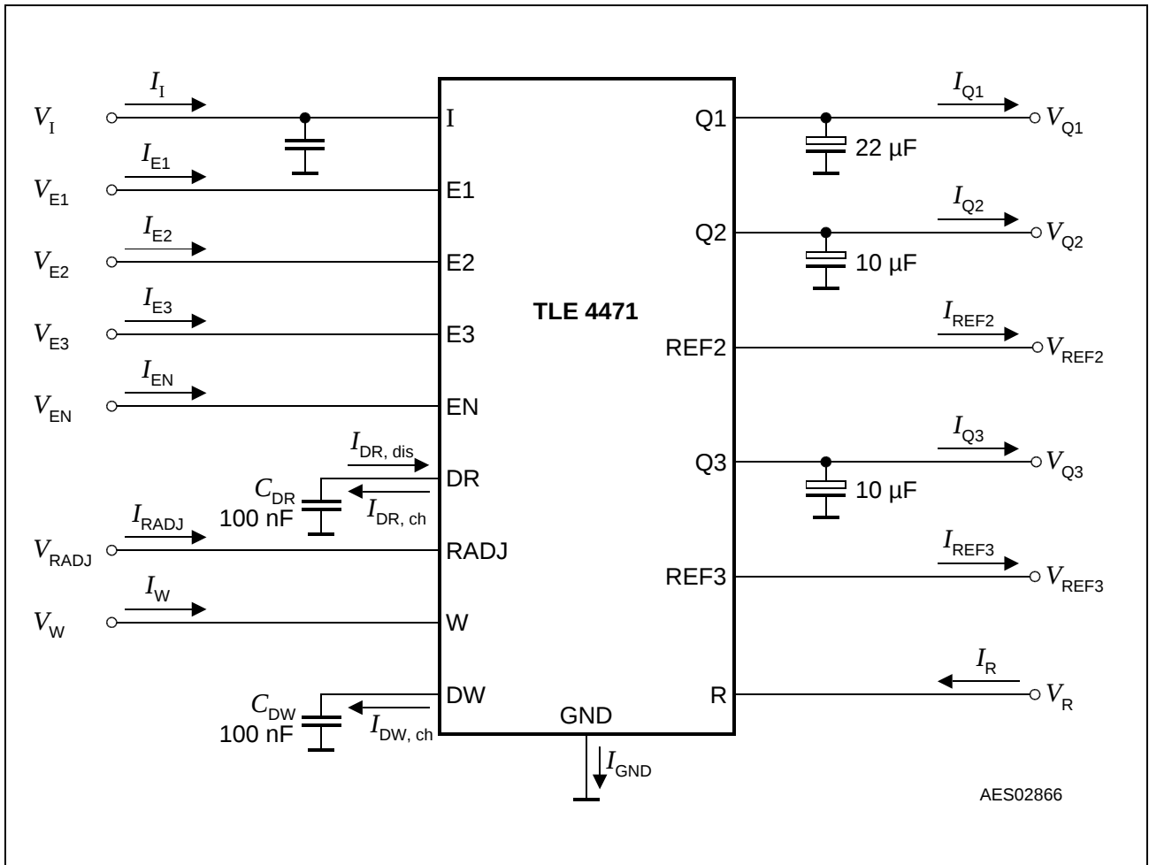
Figure 3 Measurement Circuit
