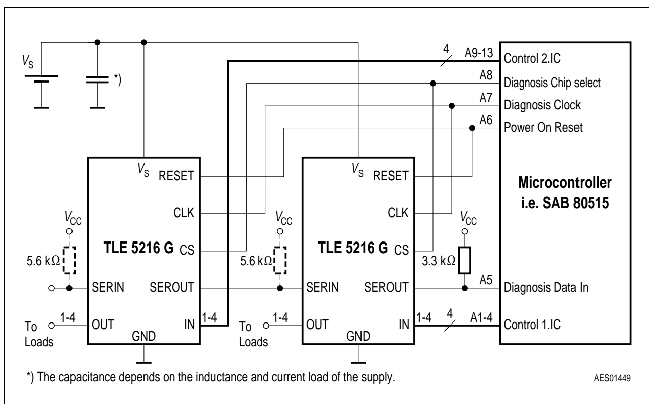
Figure 9 Application Circuit
