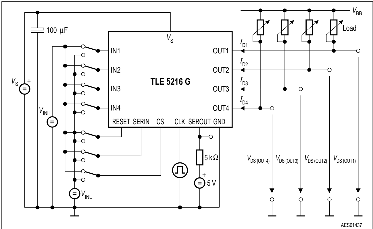
Figure 3 Test Circuit 1
