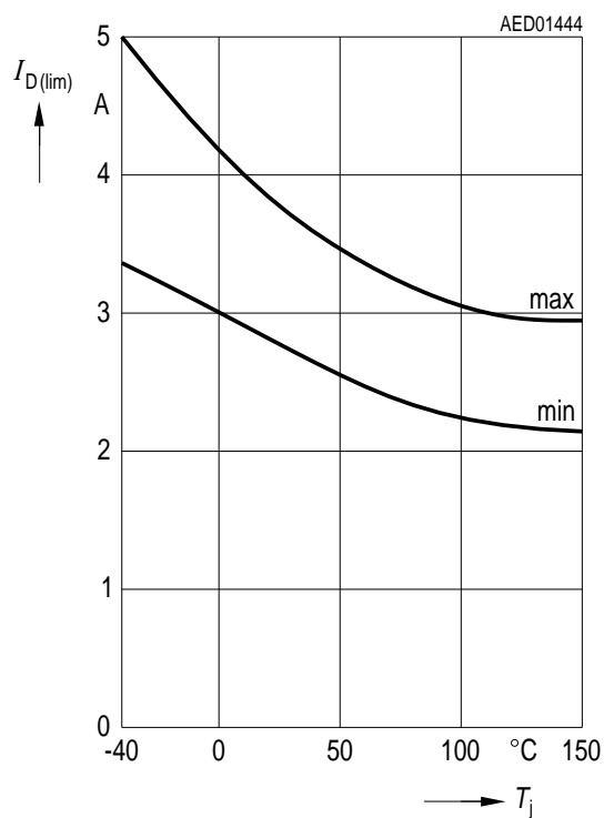
Current Limitation versus Temperature
