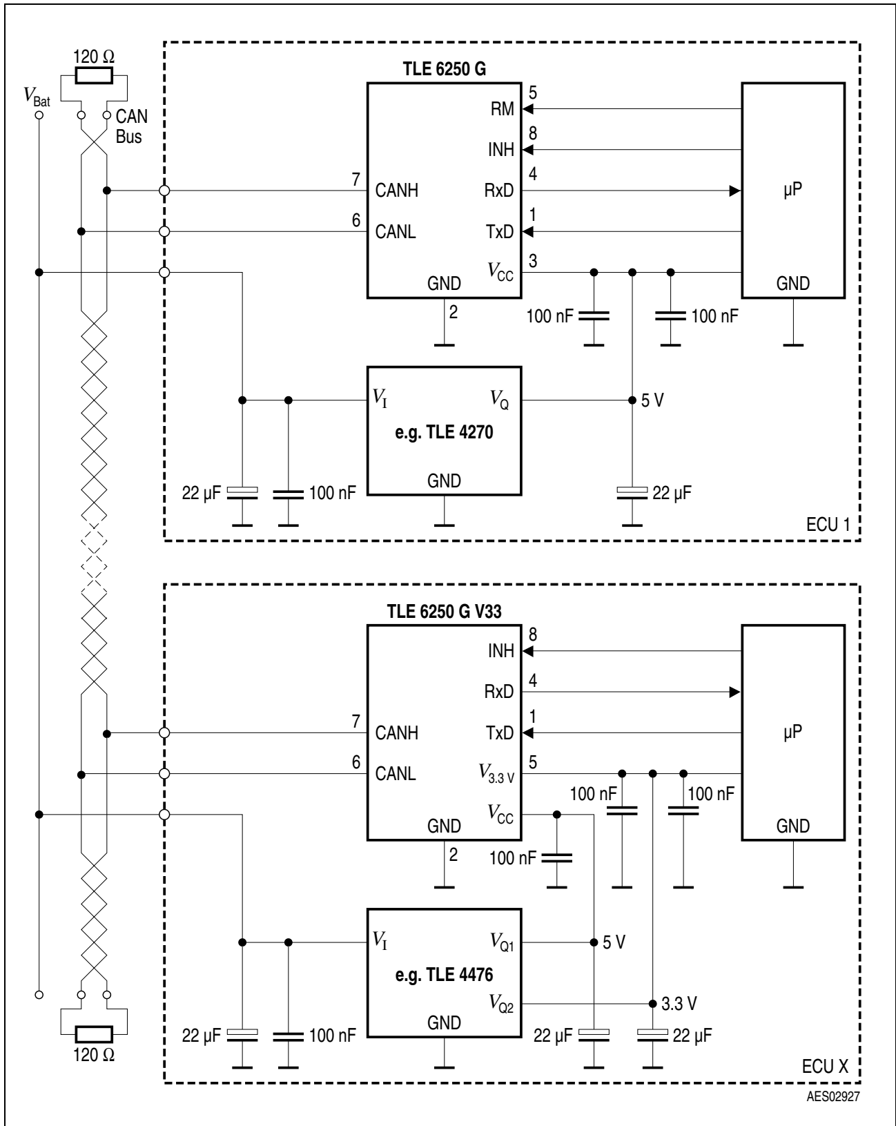
Figure 7 Application Circuit
