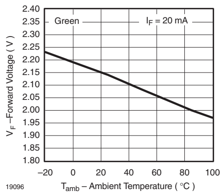
Figure 22. Forward Voltage vs. Ambient Temperature
