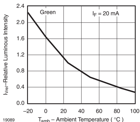
Figure 21. Relative Luminous Intensity vs. Amb. Temperature
