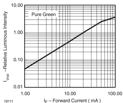
Figure 19. Relative Luminous Intensity vs. Forward Current
