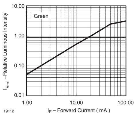
Figure 24. Relative Luminous Intensity vs. Forward Current
