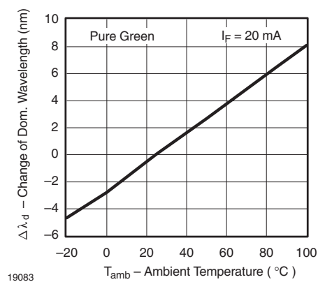
Figure 15. Change of Dominant Wavelength vs. Ambient Temperature
