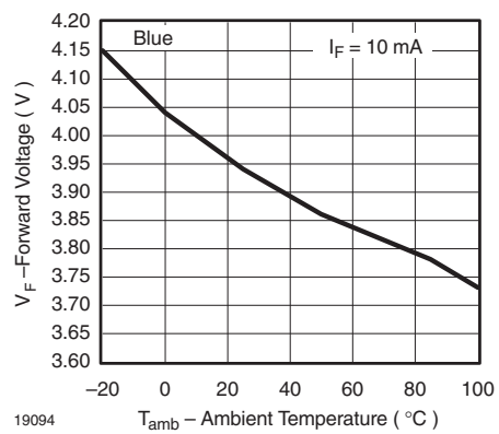
Figure 12. Forward Voltage vs. Ambient Temperature
