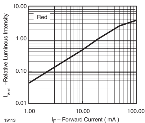
Figure 34. Relative Luminous Intensity vs. Forward Current
