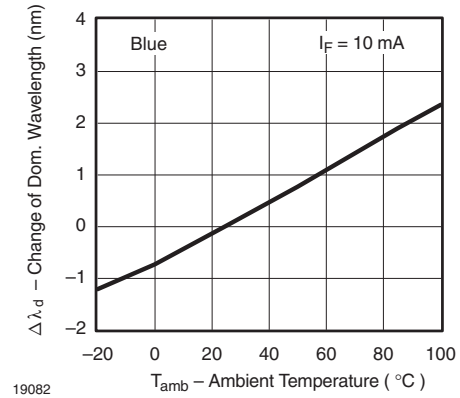
Figure 10. Change of Dominant Wavelength vs. Ambient Temperature
