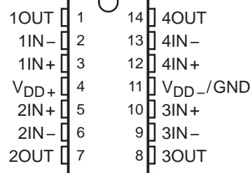
TLV2254I, TLV2254AI, TLV2254Q, TLV2254AQ . . . D OR N PACKAGE TLV2254M, TLV2254AM . . . J OR W PACKAGE (TOP VIEW)
