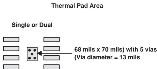
Figure 28. PowerPAD PCB Etch and Via Pattern
