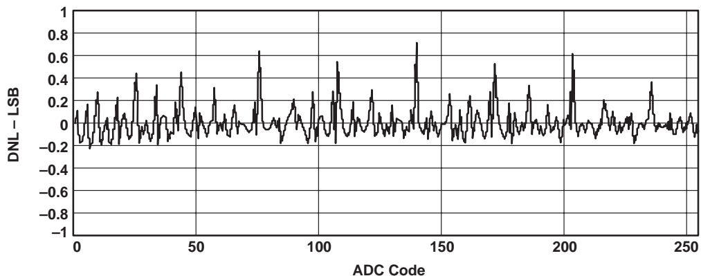
Figure 2. DNL vs Input Code At 80 MSPS (With External Reference, PW Package)
