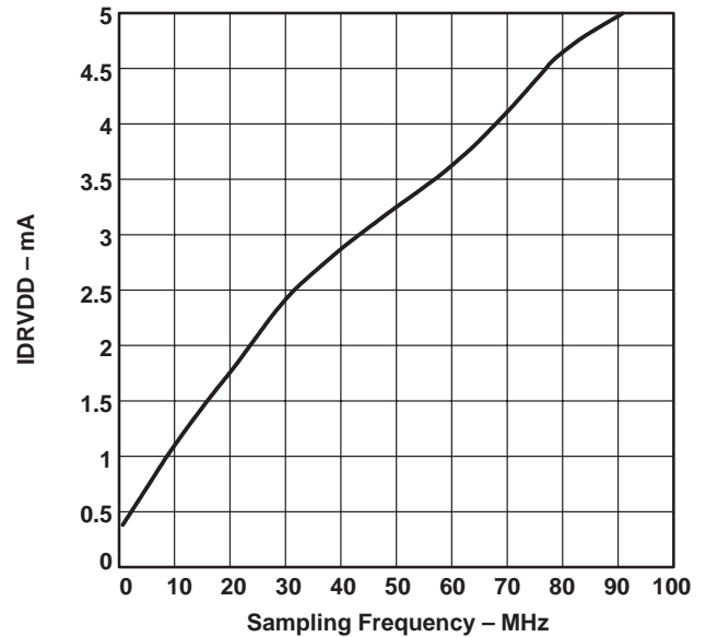
Figure 10. IDR_VDD vs f_{CLK} At V_{IN} = 1 MHz, -1 dBFS
