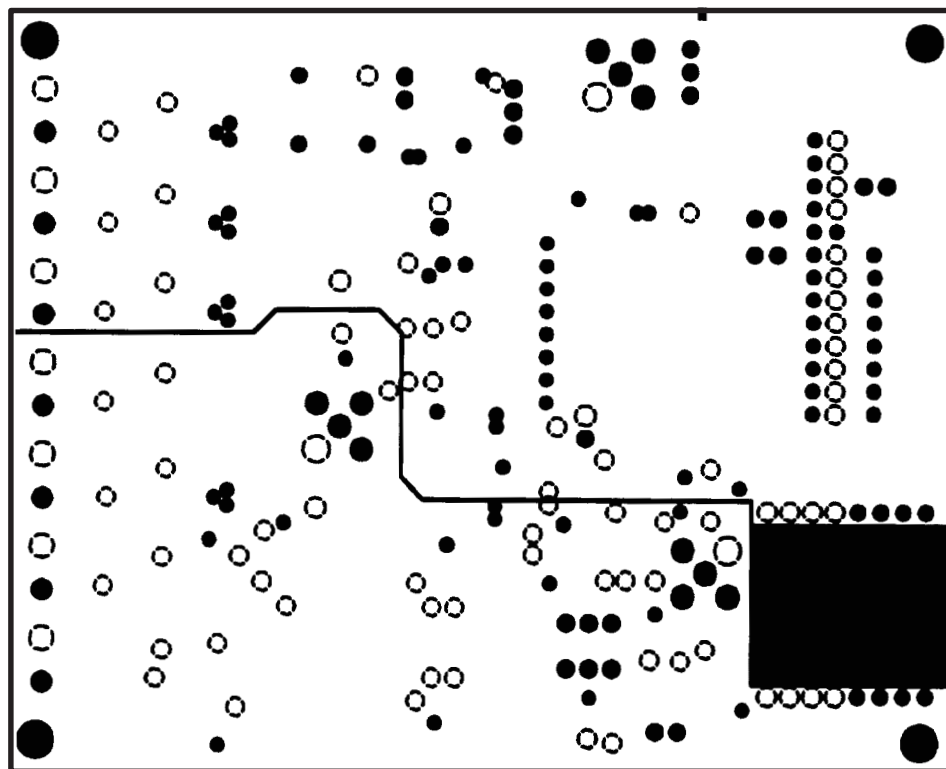
Internal Plane 1
