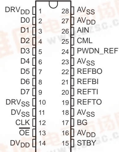
DW OR PW PACKAGE (TOP VIEW)
