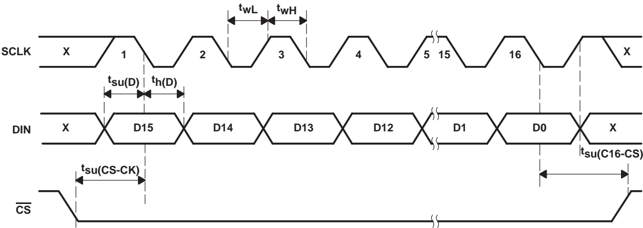
Figure 1. Timing Diagram
