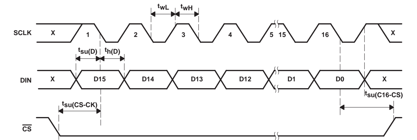
Figure 1. Timing Diagram
