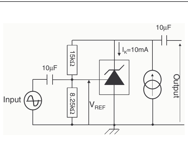
Figure 6. Test circuit for phase margin and voltage gain
