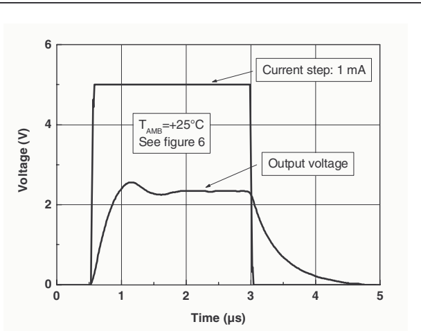
Figure 20. Pulse response for I_K = 1 mA
