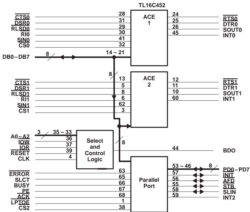
TL16C452 functional block diagram
