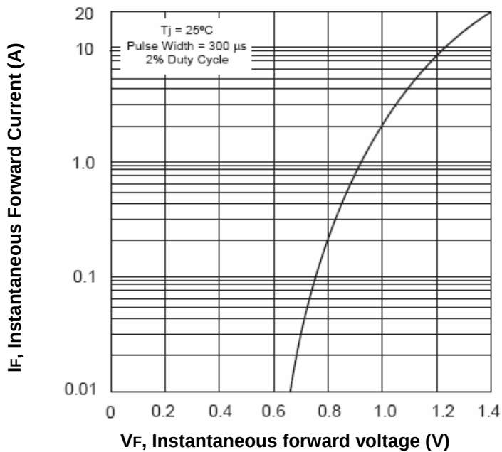
Fig.3-Typical Forward Characteristic per element
