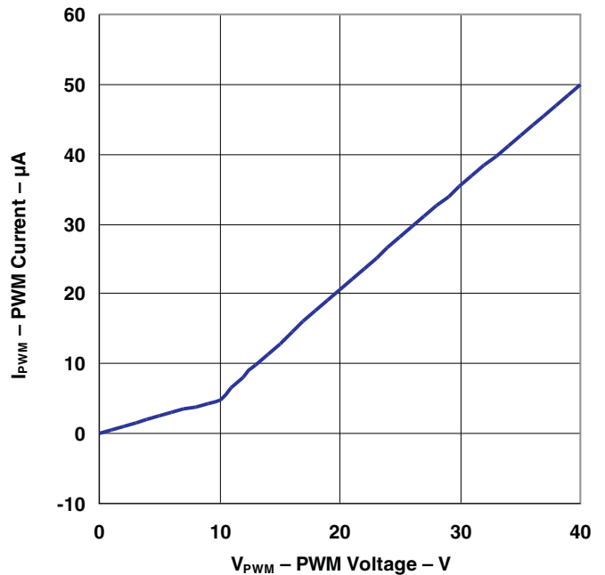
Figure 4. PWM Pin Input Current vs PWM Voltage
