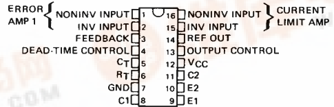
TL494I, TL494C . . . D, J, OR N PACKAGE (TOP VIEW)
