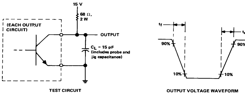
FIGURE 3. COMMON-EMITTER CONFIGURATION
