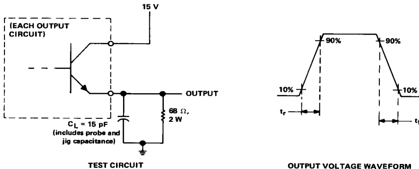
FIGURE 4. EMITTER-FOLLOWER CONFIGURATION
