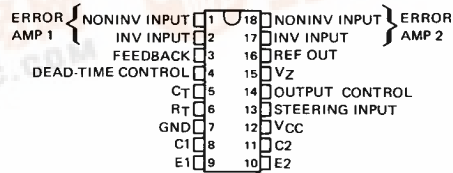
TL495C . . . N PACKAGE (TOP VIEW)
