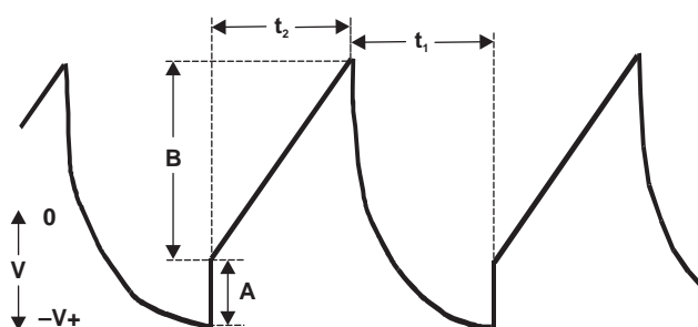
Figure 4. Output Ripple
