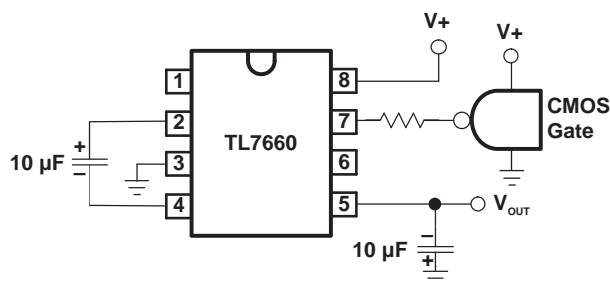
Figure 7. External Clocking
