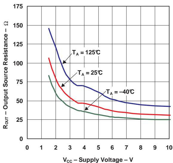
OUTPUT RESISTANCE vs SUPPLY VOLTAGE
