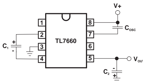
Figure 8. Lowering Oscillator Frequency
