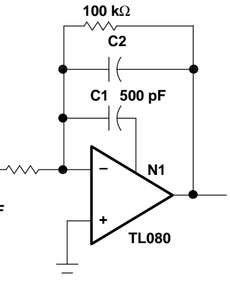
Figure 3. Feed-Forward Compensation
