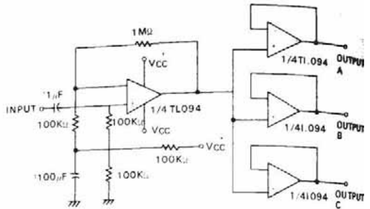
FIGURE 10-AUDIO DISTRIBUTION AMPLIFIER
