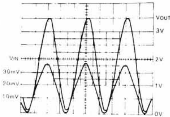
FIGURE 9 SINGLE SUPPLY NON-INVERTING AMP AND WAVE FORM
