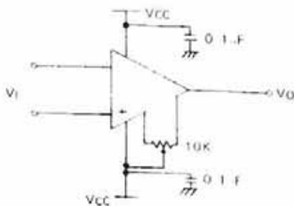
FIGURE 12 TL091 OFFSET ADJUSTMENT
