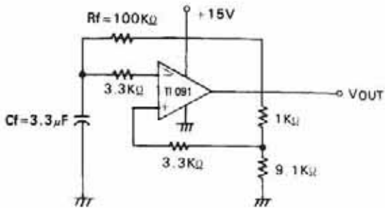
FIGURE 16-0 5Hz SQUARE-WAVE OSCILLATOR
