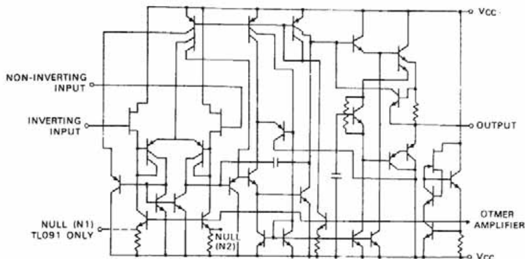
SCHEMATIC (EACH AMPLIFIER)
