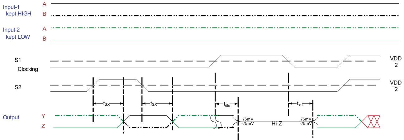
Figure 6. TMS Outputs Control Timing Definitions
