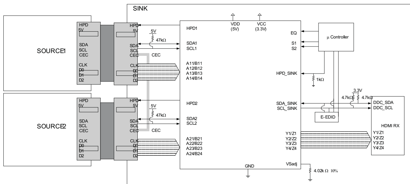
Figure 18. Two-Port HDMI Enabled DTV with TMS250 – CEC Commands Passing Through
