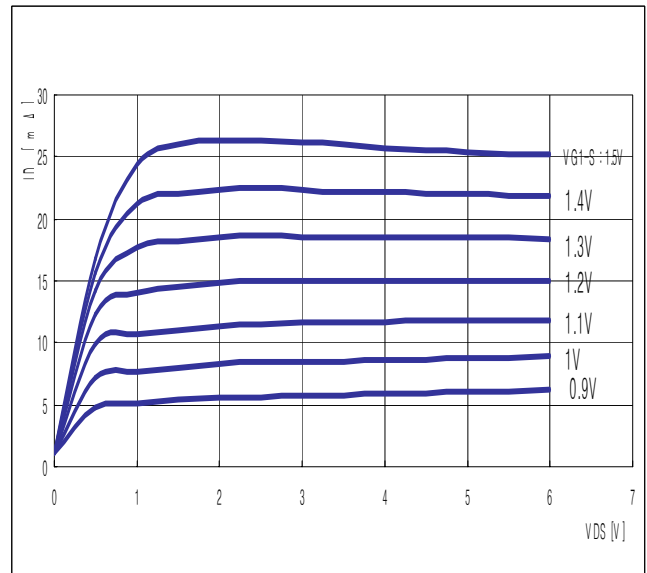
Fig3. Output characteristics
