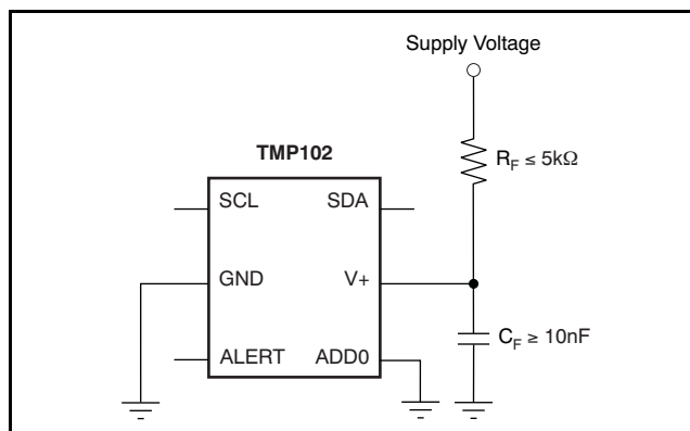
Figure 11. Noise Reduction
