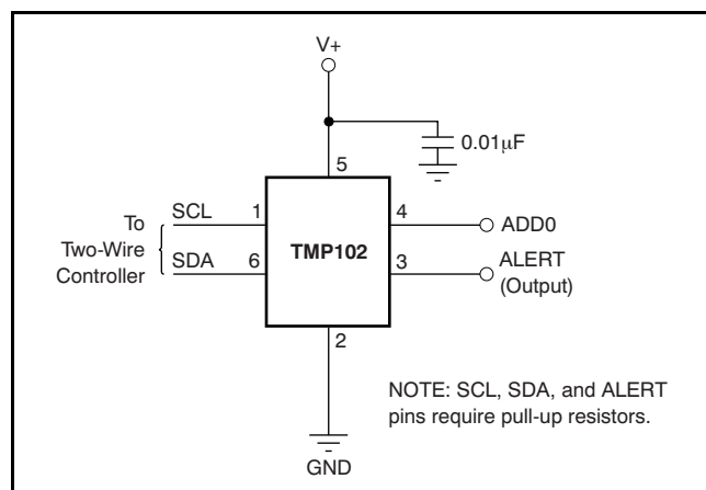
Figure 7. Typical Connections
