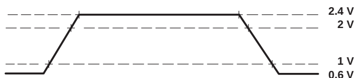
Figure 6. TTL-Level Outputs
