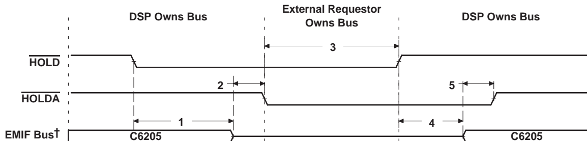
Figure 27. \overline{\text{HOLD}}/\overline{\text{HOLDA}} Timing
