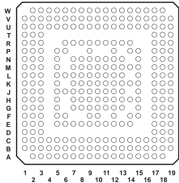
GHK and ZHK 288-PIN BALL GRID ARRAY (BGA) PACKAGES (BOTTOM VIEW)
