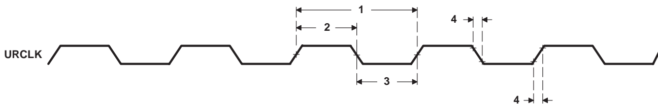
Figure 58. URCLK Timing
