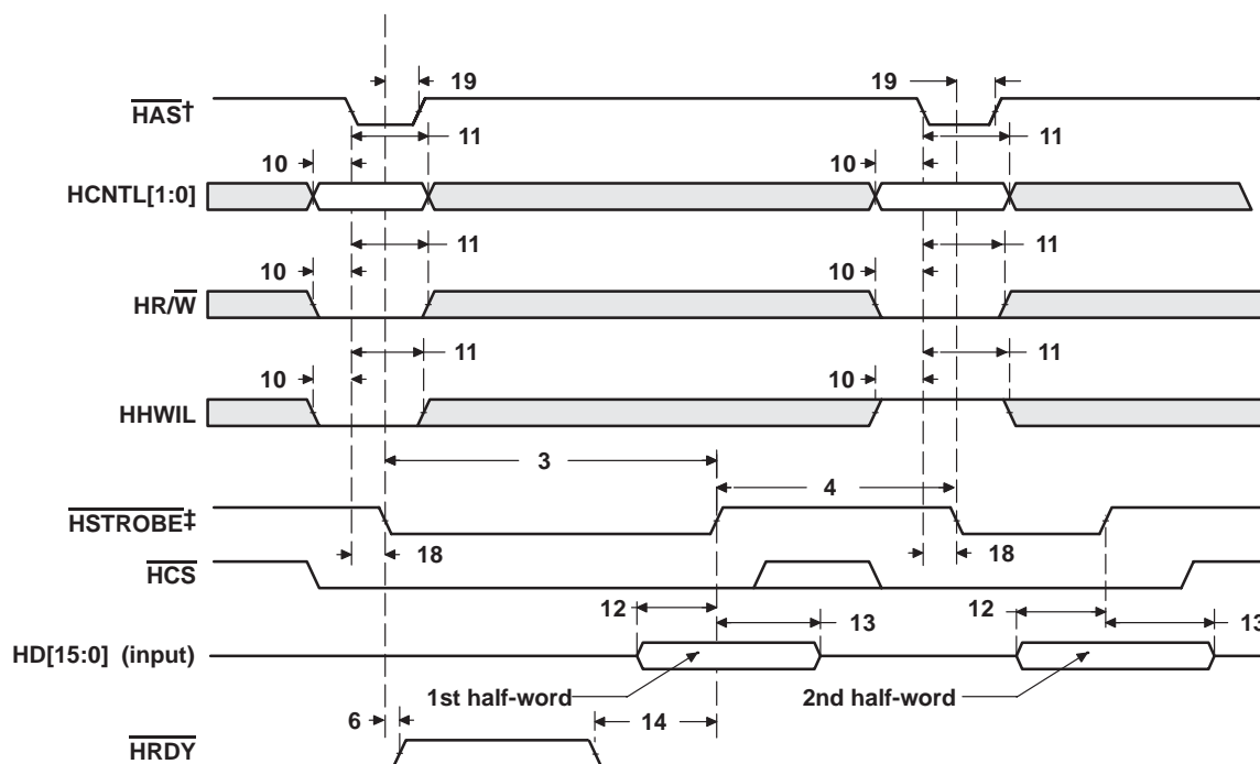
Figure 42. HPI16 Write Timing ( \overline{HAS} Used)
