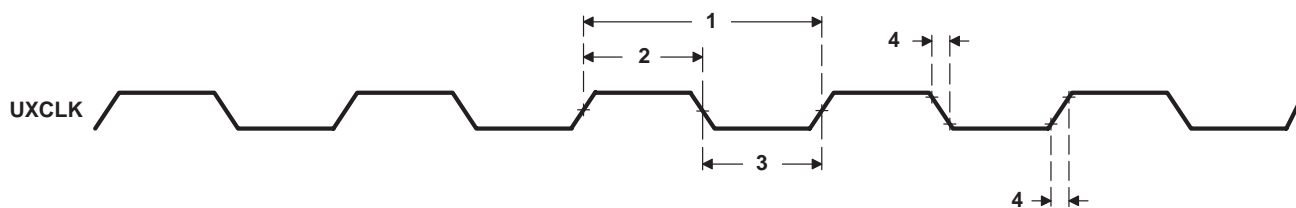
Figure 57. UXCLK Timing
