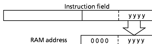
Figure 2-5. Addressing mode
