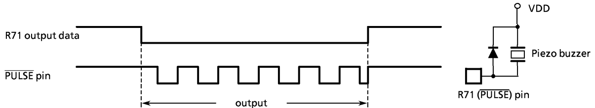
Figure 3-17. Circuit Example of Buzzer Pulse and Timing
