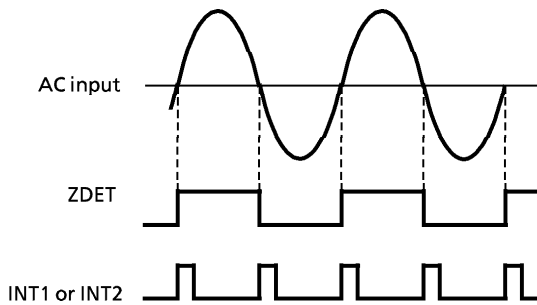
Figure 3-20. Detection Signal
