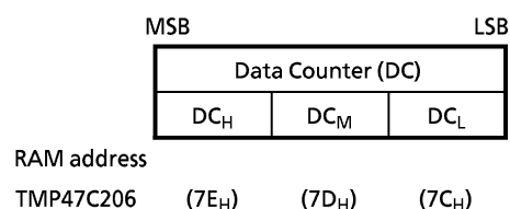
Figure 2-7. Data Counter
