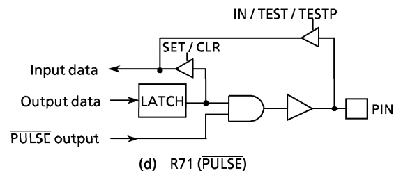
Figure 3-3. Ports R4, R5 and R7
