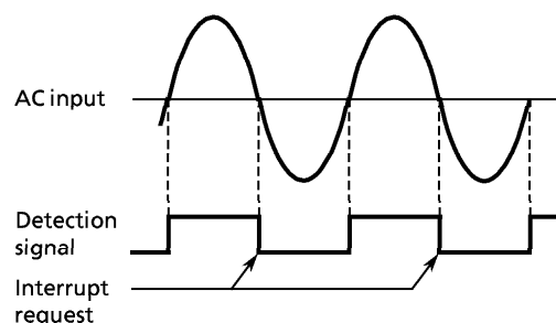
Figure 3-25. Detection Signal
