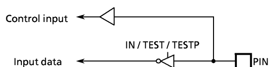
Figure 3-7. Port KE
