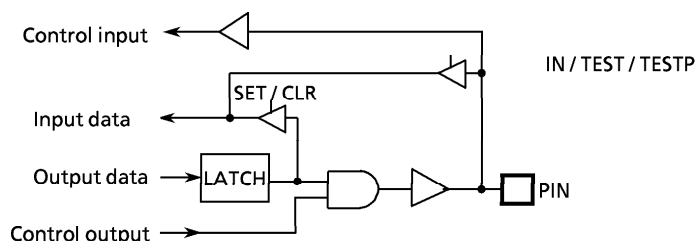
Figure 3-6. Port R9
