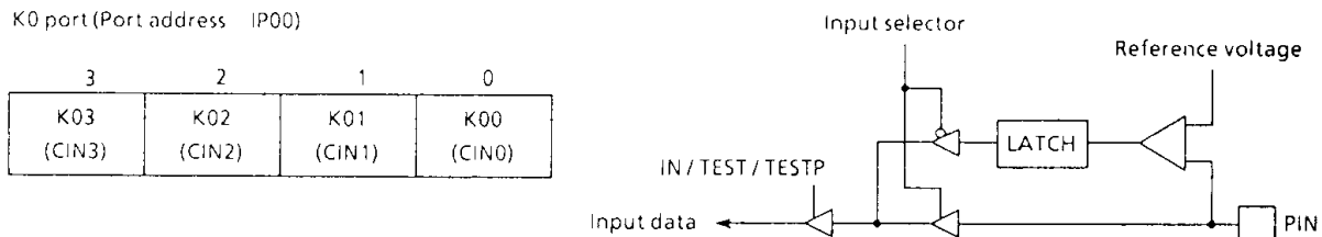
Figure 2-1. K0 port
