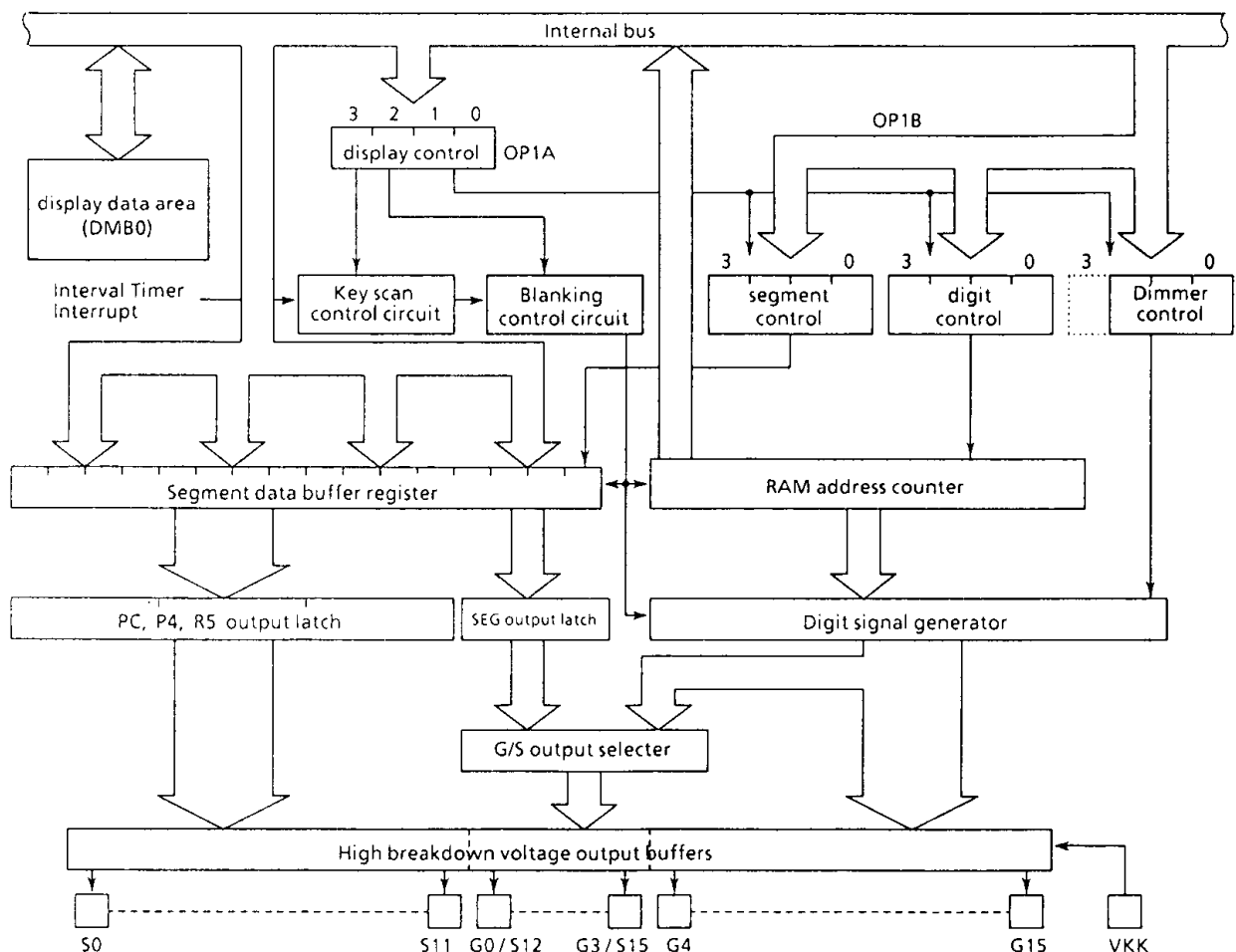
Figure 2-7. VFT drive circuit
