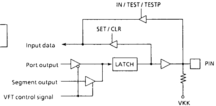
Figure 2-4. R5 port
