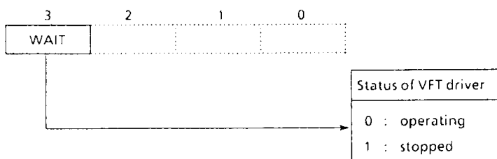
Figure 2-8. VFT driver command register, status register
