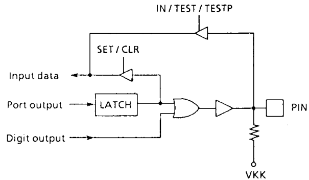
Figure 2-5. R3, RA, RB port
