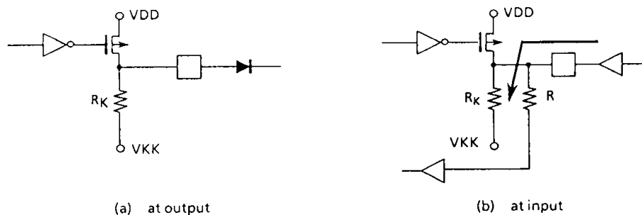
Figure 2-14. Input/Output interface
