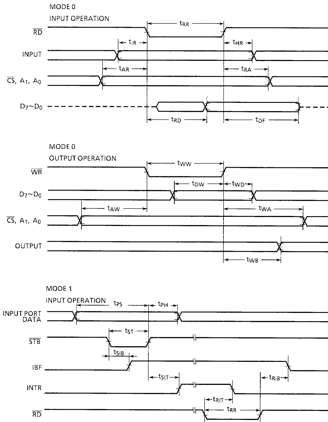
Figure 7.1 Timing diagram
