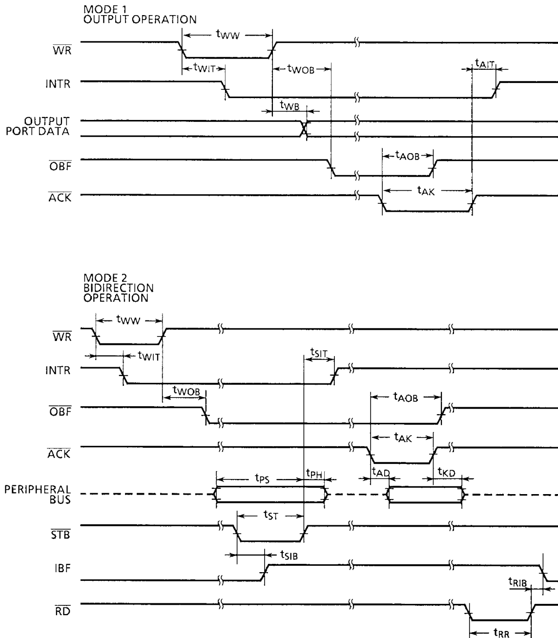
Figure 7.2 Timing Diagram
