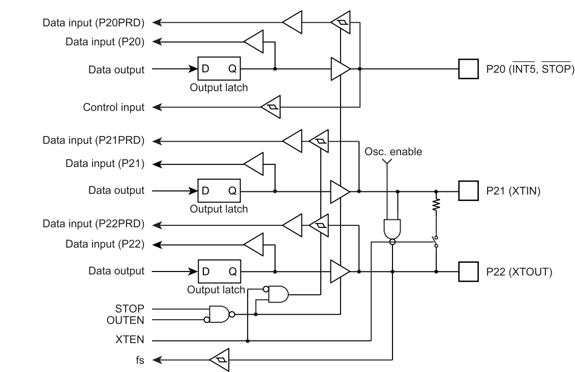
Figure 5-4 P2 Port
