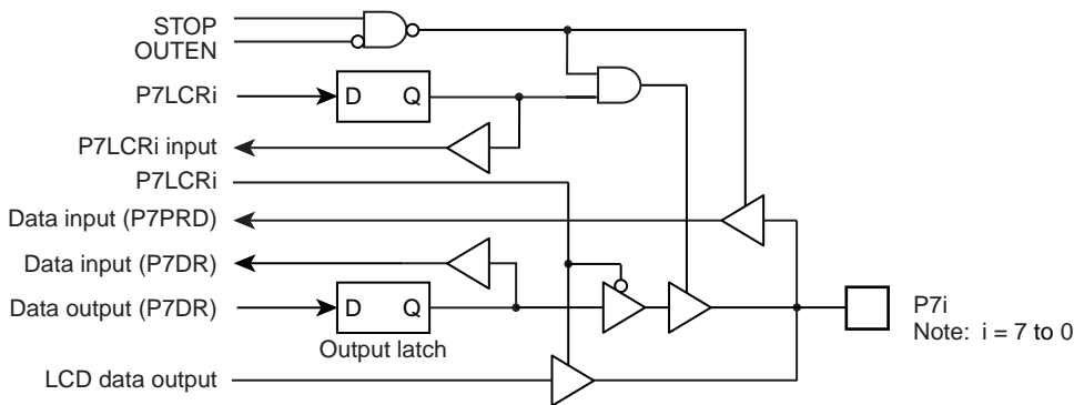
Figure 5-7 Port 7
