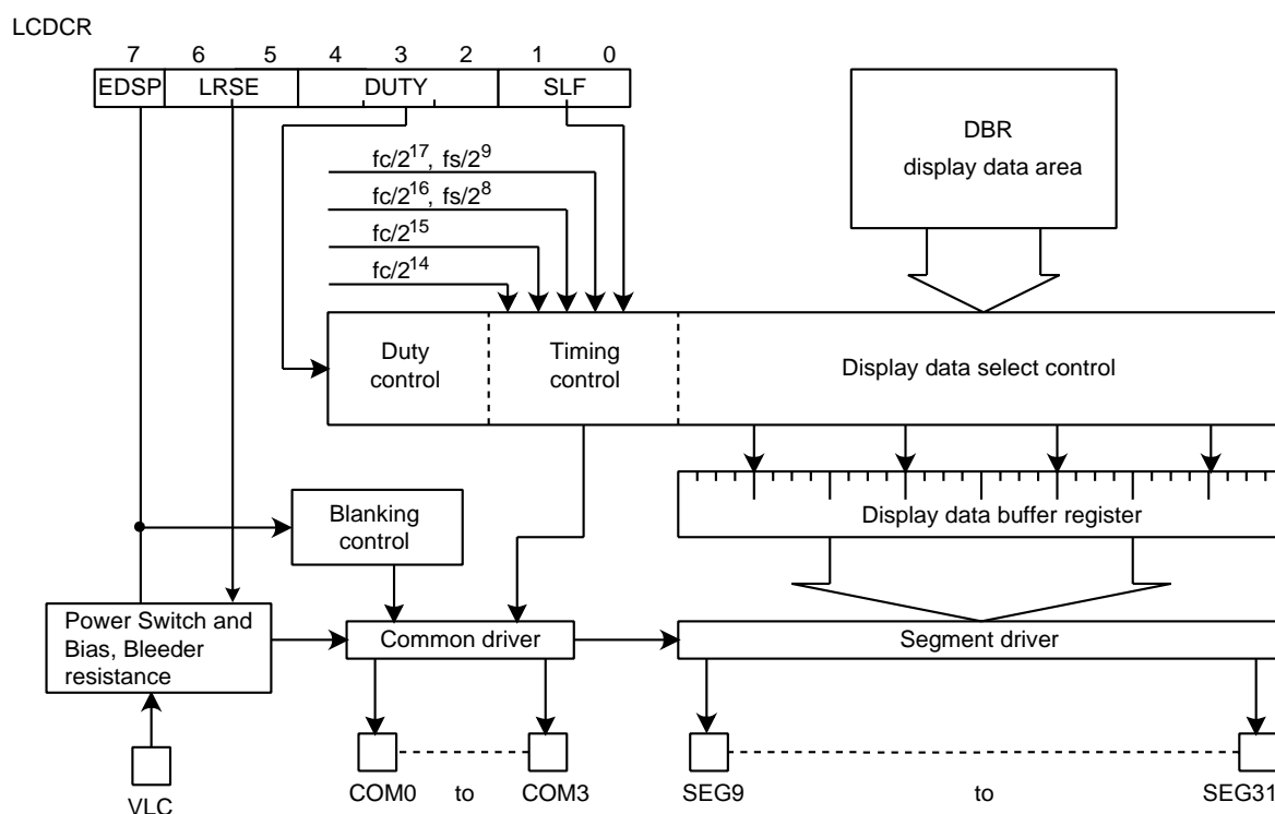
Figure 15-1 LCD Driver
