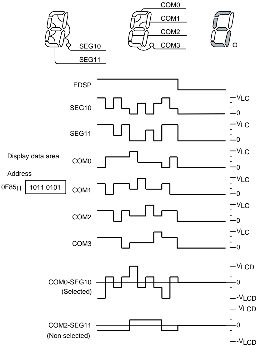
Figure 15-7 1/4 Duty (1/3 Bias) Drive
