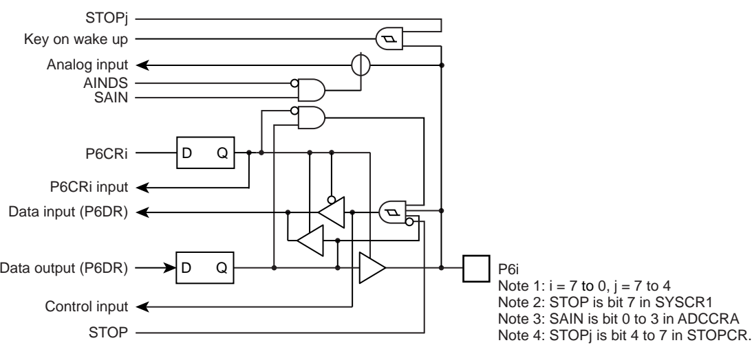
Figure 5-6 Port P6
