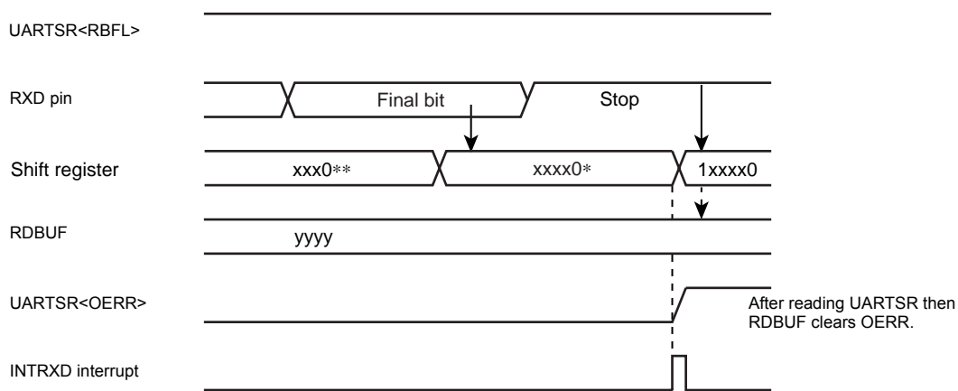
Figure 11-7 Generation of Overrun Error
