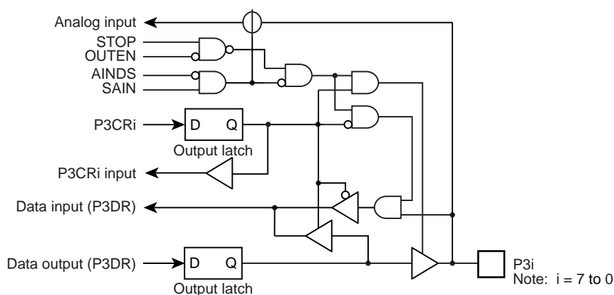
Figure 5-5 Port 3
