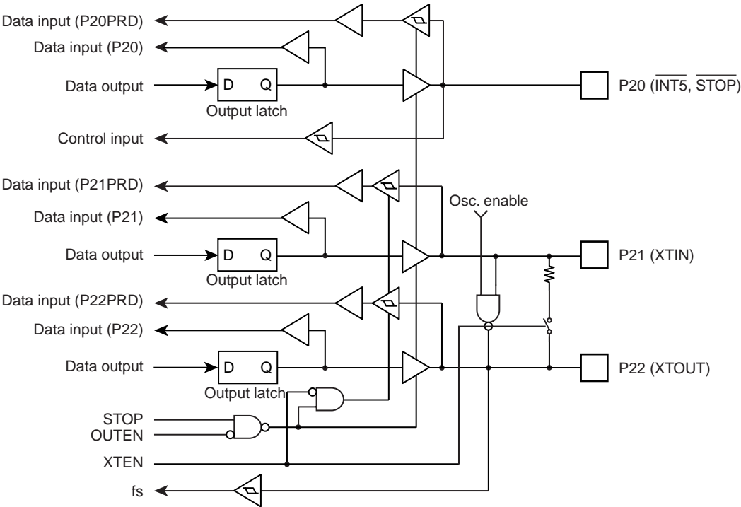
Figure 5-4 Port 2
