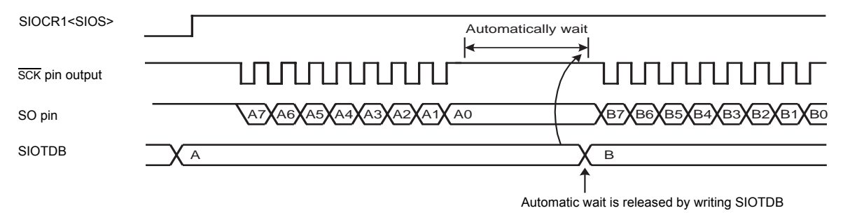
Figure 9-2 Automatic-wait Function (Example of transmit mode)
