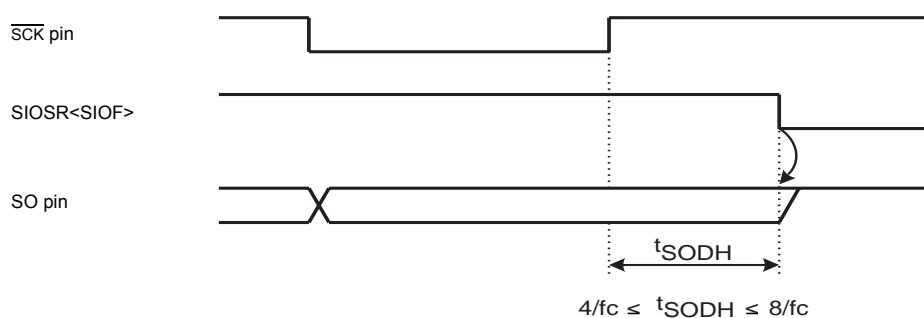
Figure 9-8 Hold Time of the End of Transmit Mode
