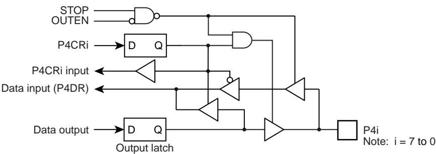
Figure 5-6 Port P4
