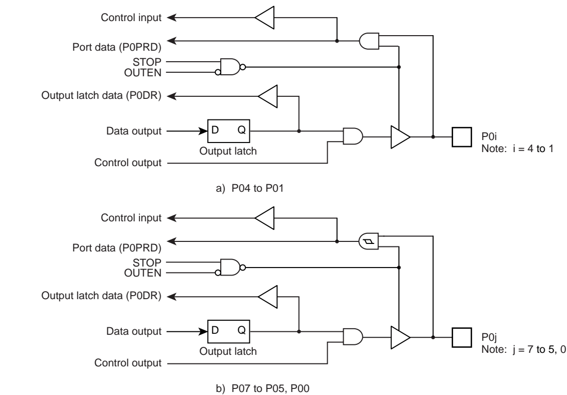
Figure 5-2 Port 0
