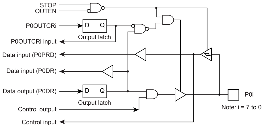
Figure 5-2 P0 Port
