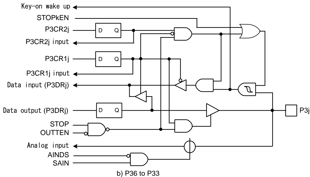
Figure 5-5 Port 3
