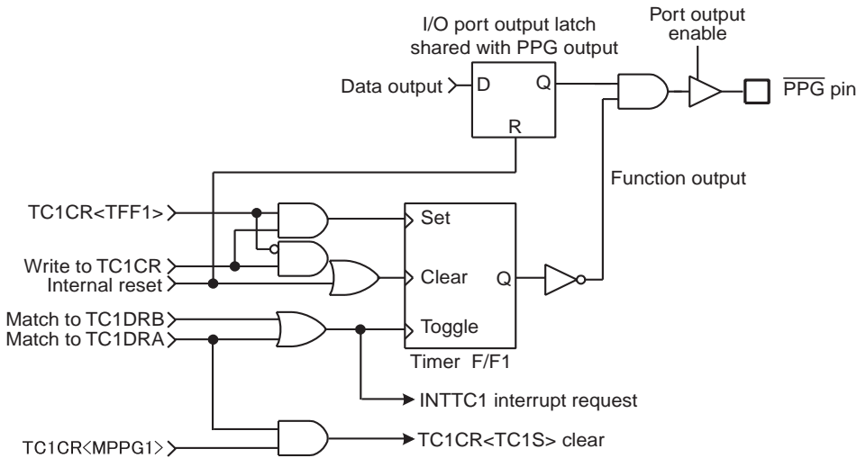
Figure 10-7 \overline{\text{PPG}} Output
