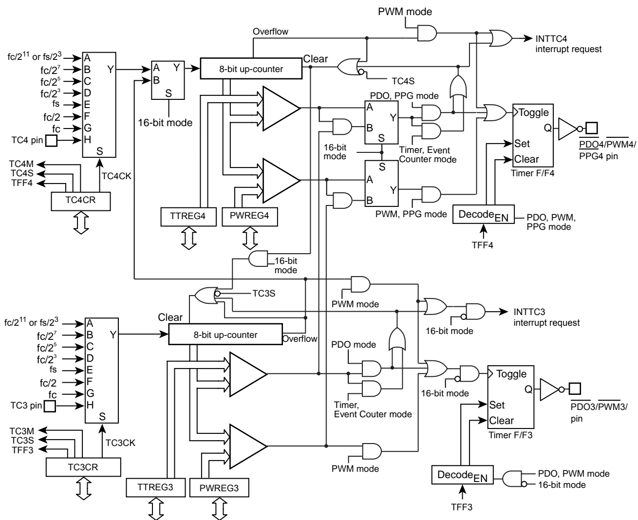
Figure 11-1 8-Bit TimerCounter 3, 4
