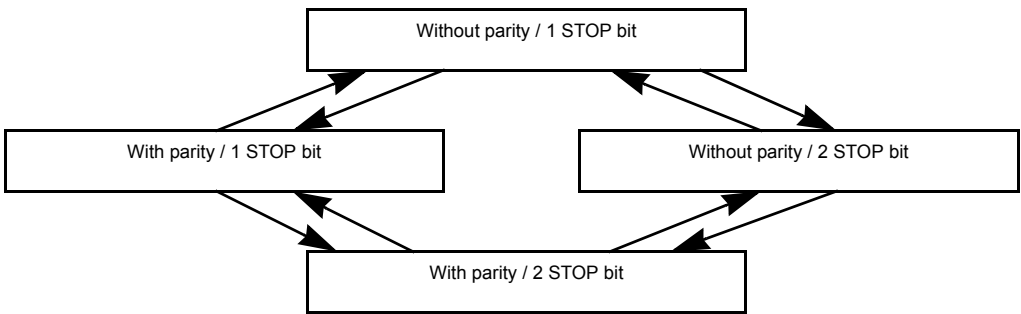
Figure 13-3 Caution on Changing Transfer Data Format
