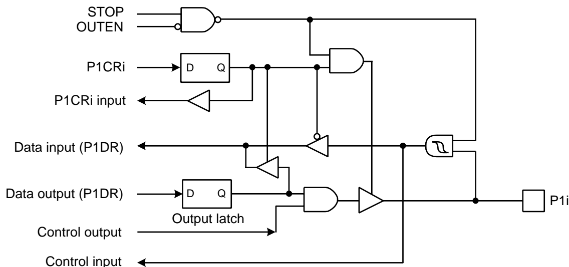
Figure 5-3 Port 1
