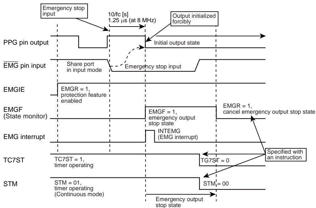
Figure 9-23 Timing between EMG Pin Input being Detected and PPG Outputs being Disabled
