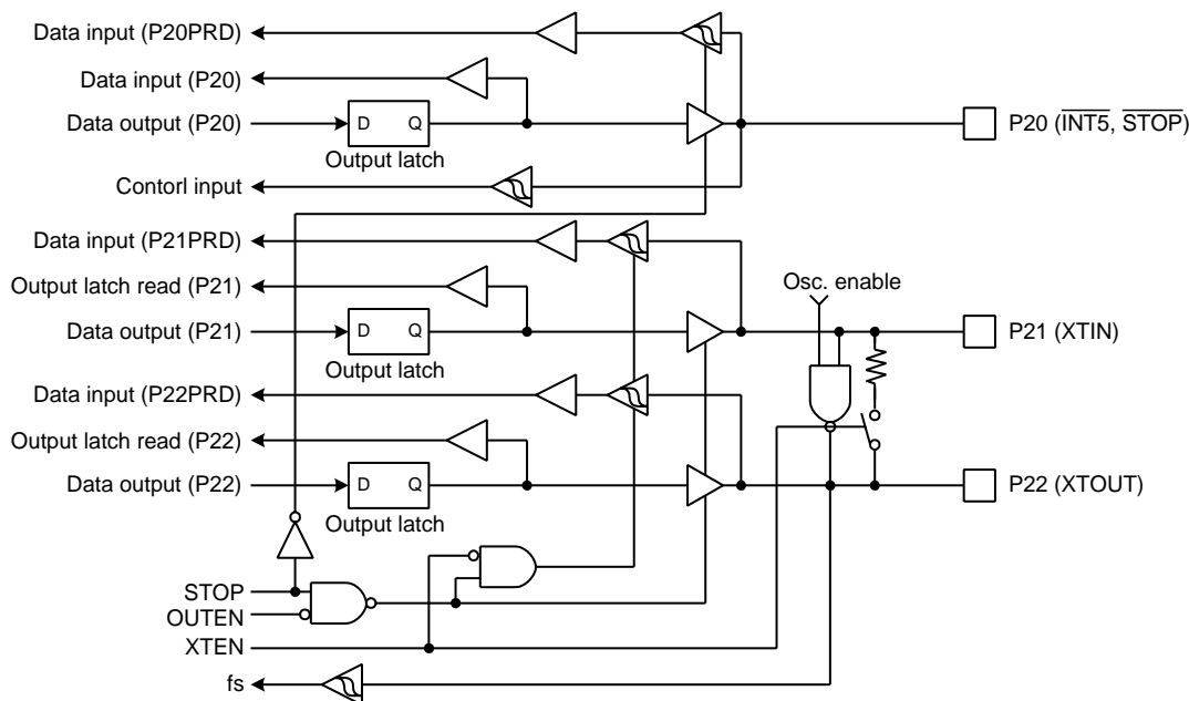
Figure 5-4 Port 2
