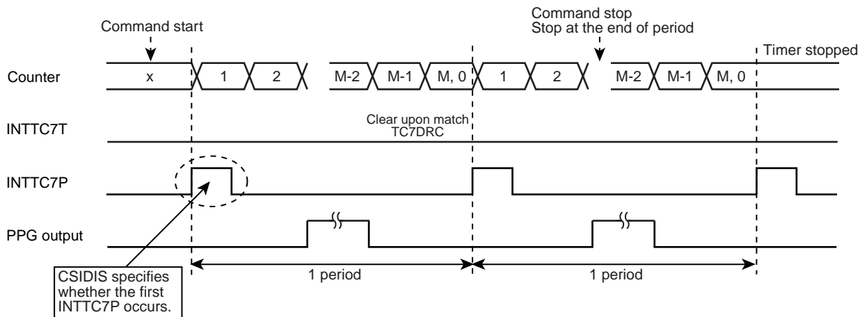
Figure 9-21 Period Interrupt
