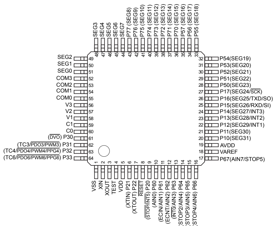
Figure 1-1 Pin Assignment
