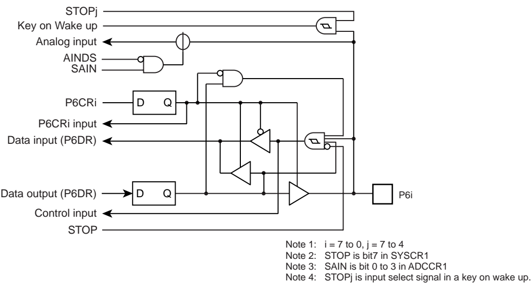
Figure 5-6 Port 6
