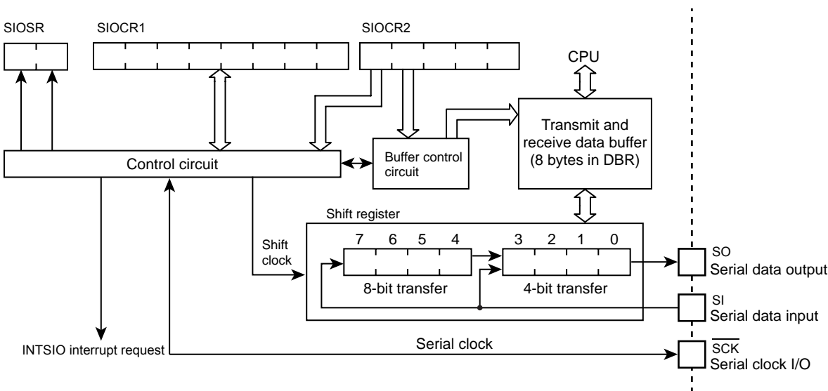
Figure 11-1 Serial Interface
