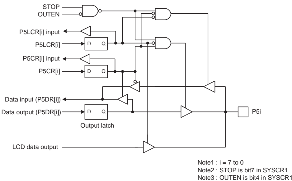
Figure 5-5 Port 5
