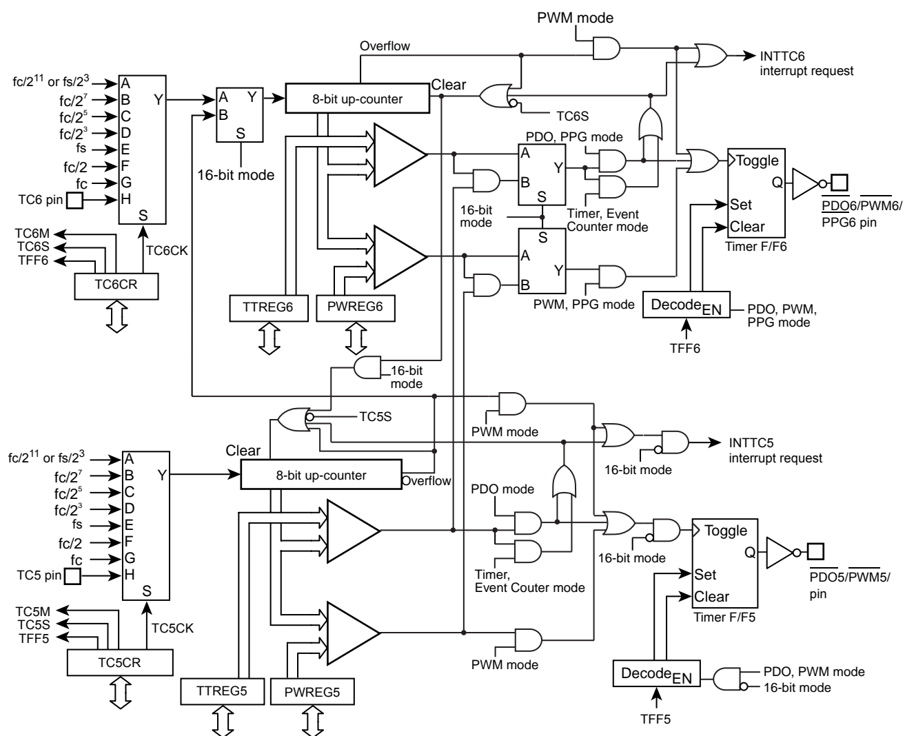
Figure 9-1 8-Bit TimerCounter 5, 6
