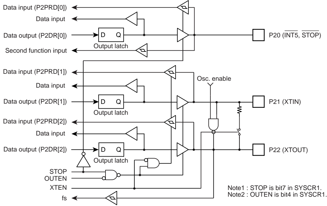
Figure 5-3 Port 2
