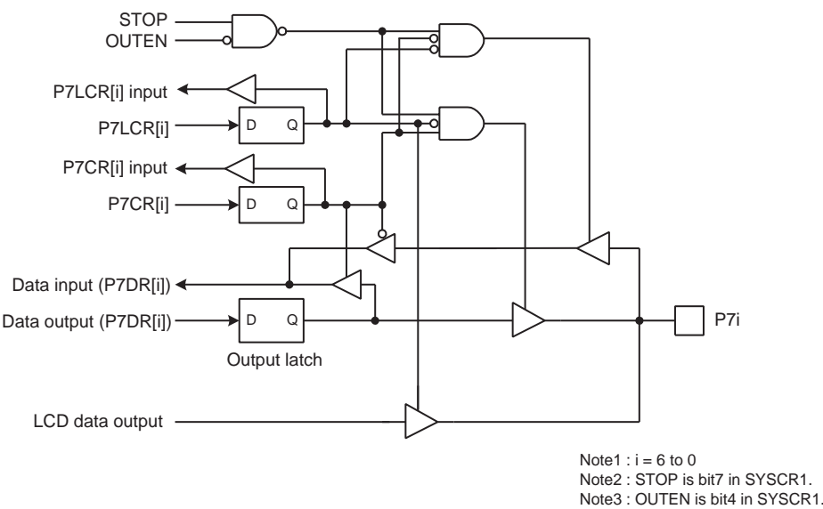
Figure 5-7 Port 7
