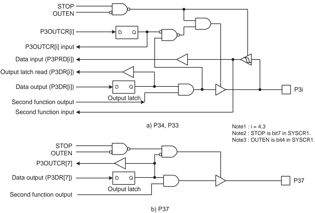
Figure 5-4 Port 3
