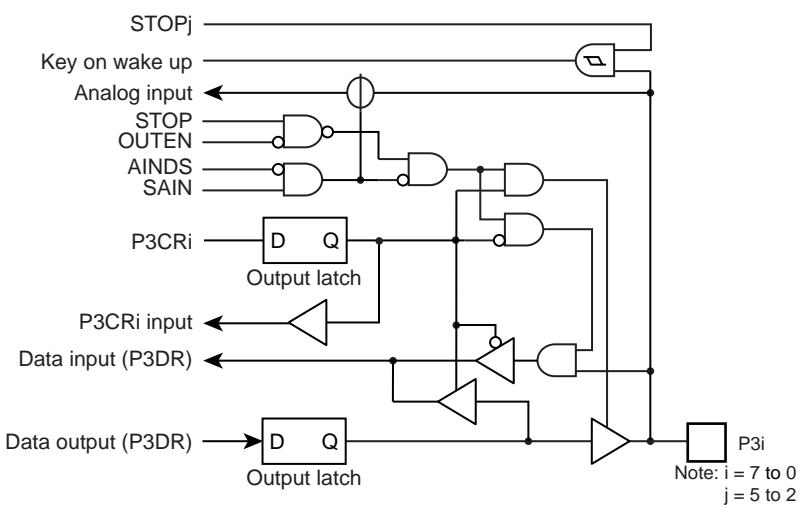
Figure 5-5 Port P3
