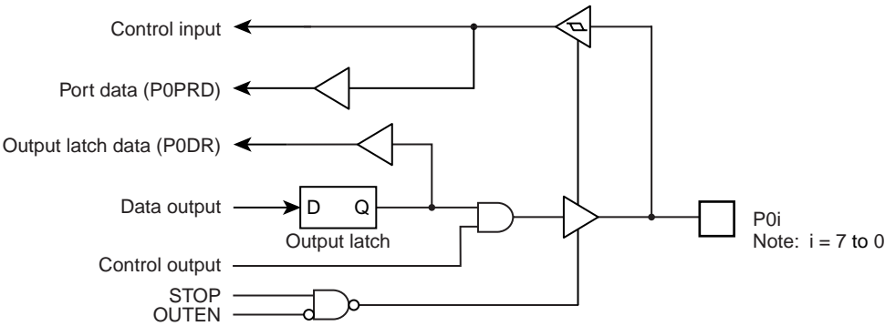
Figure 5-2 Port 0
