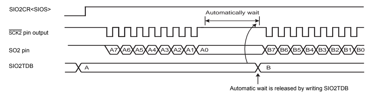
Figure 15-2 Automatic-wait Function (Example of transmit mode)
