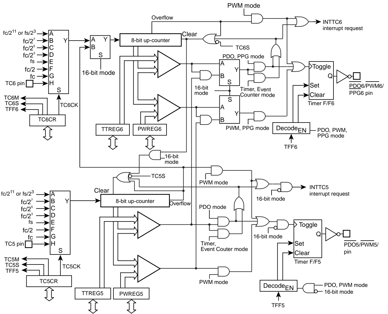
Figure 10-1 8-Bit TimerCounter 5, 6
