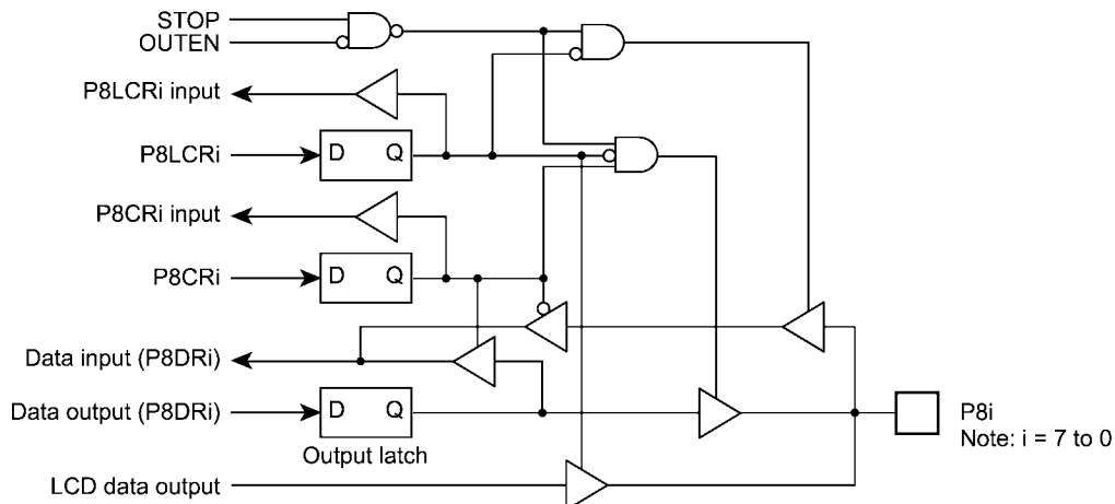
Figure 5-8 Port P8
