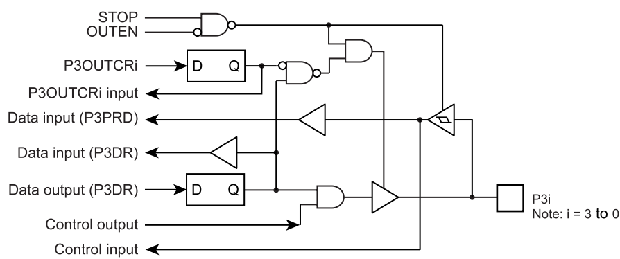
Figure 5-4 Port P3
