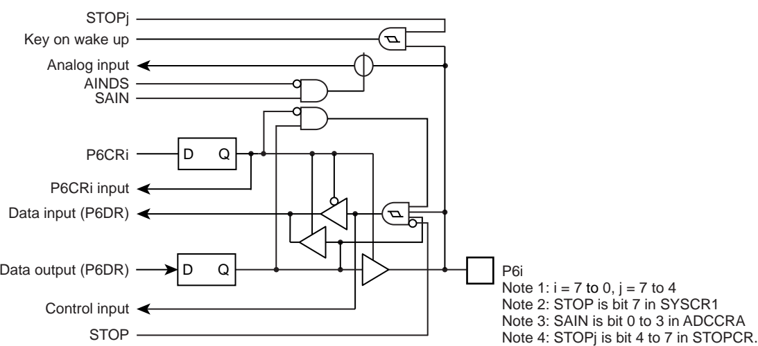
Figure 5-6 Port P6
