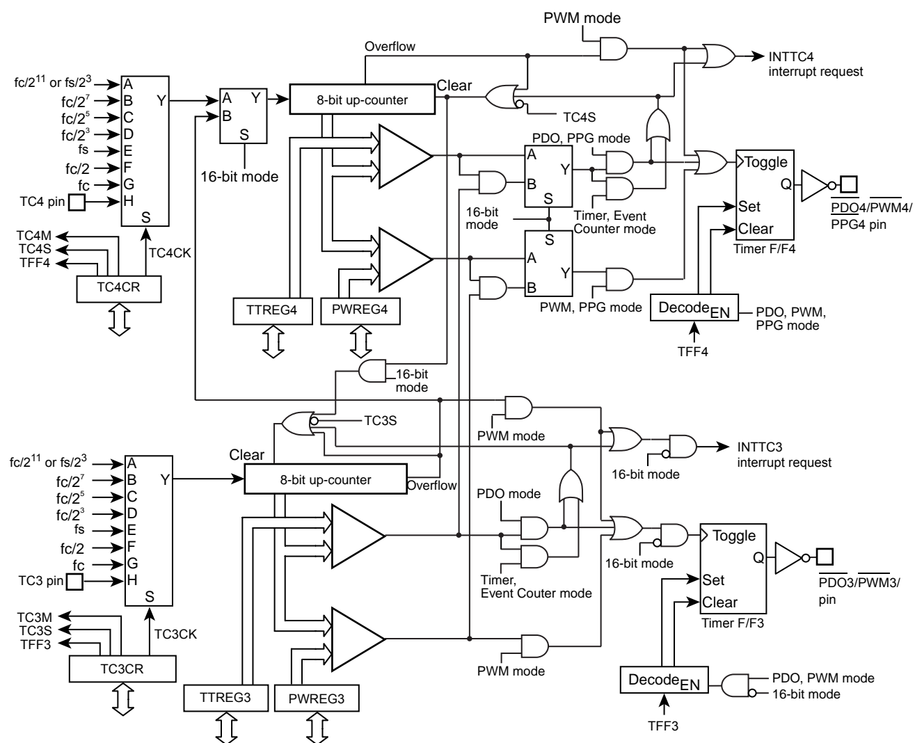
Figure 9-1 8-Bit TimerCounter 3, 4
