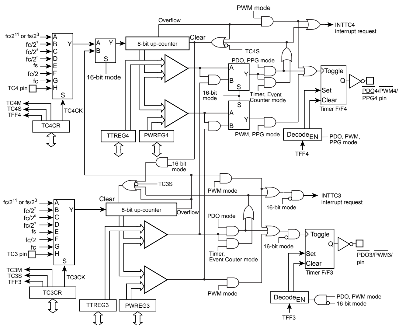
Figure 10-1 8-Bit TimerCounter 3, 4
