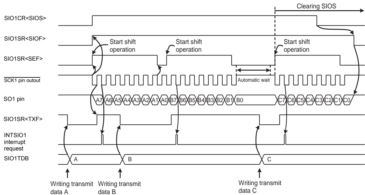
Figure 14-6 Example of Internal Clock and MSB Transmit Mode
