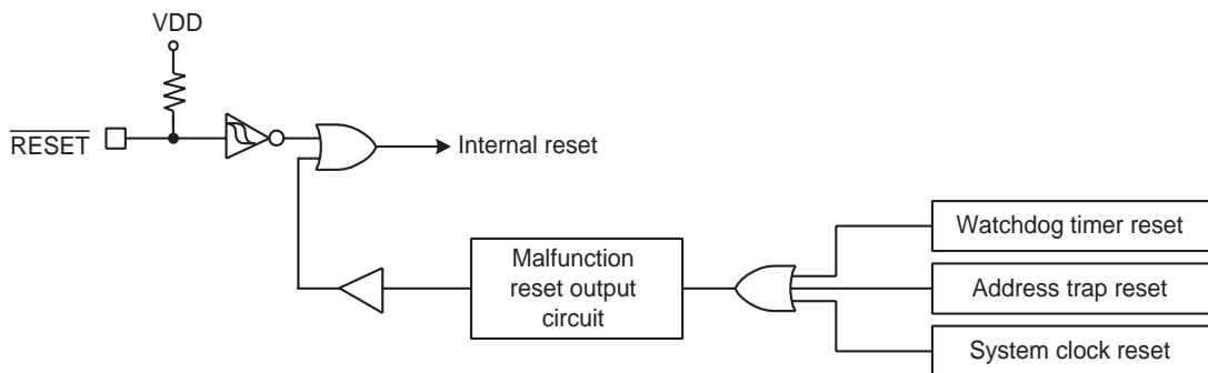
Figure 2-15 Reset Circuit
