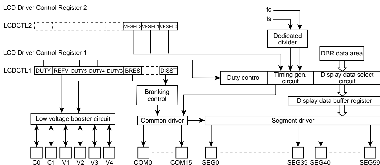
Figure 16-1 LCD Driver Block Diagram
