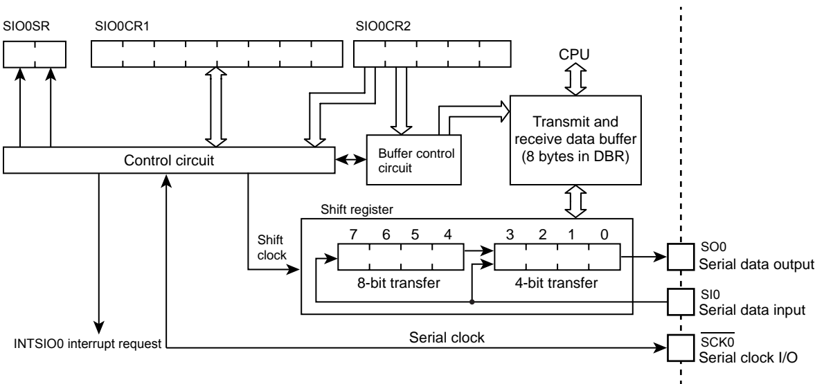
Figure 12-1 Serial Interface
