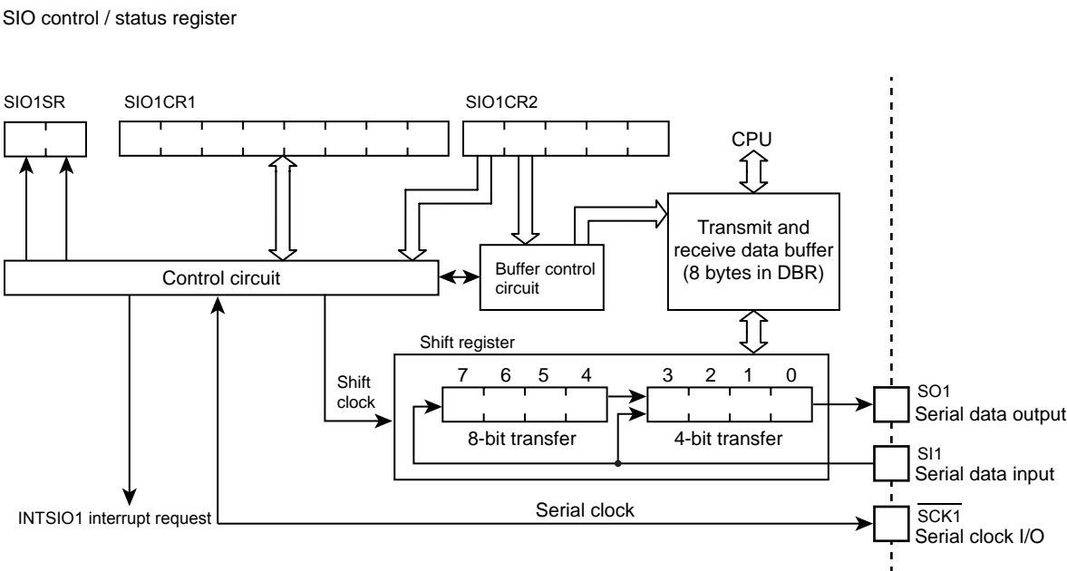
Figure 13-1 Serial Interface
