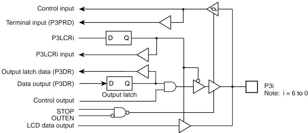
Figure 5-4 Port 3
