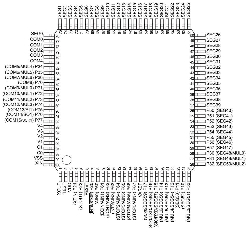
Figure 1-1 Pin Assignment
