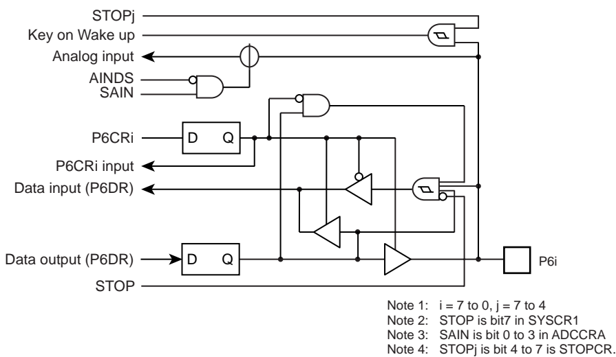
Figure 5-6 Port 6
