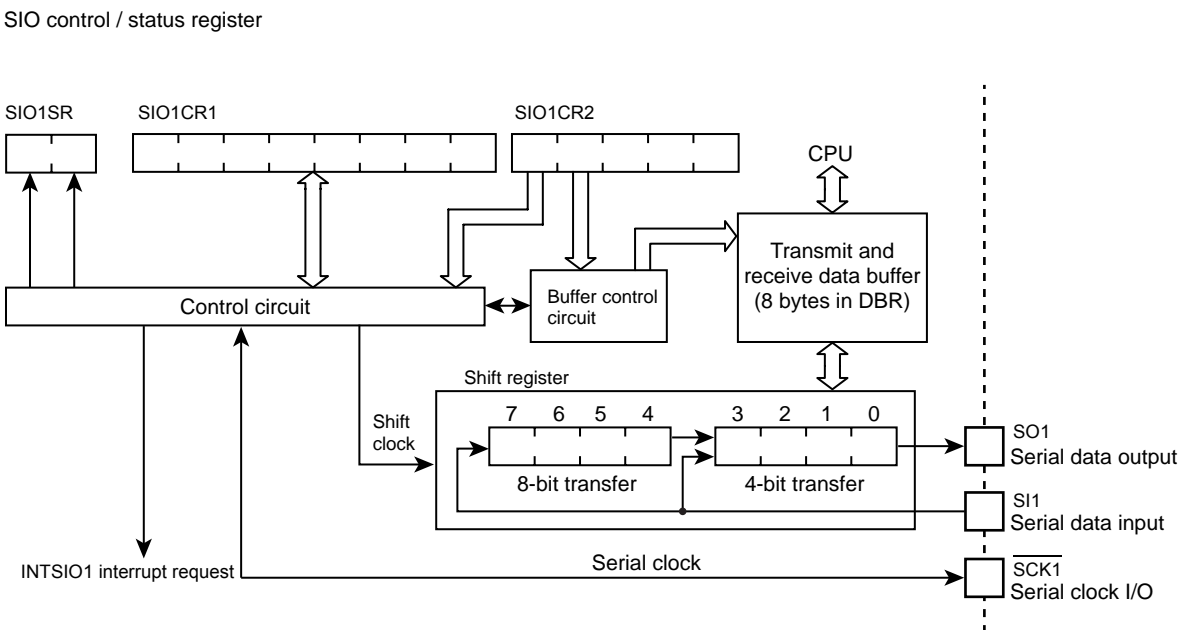
Figure 13-1 Serial Interface
