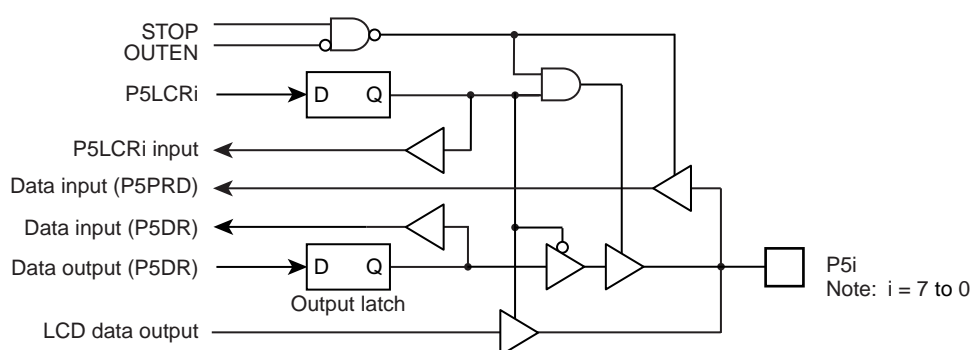
Figure 5-5 Port 5
