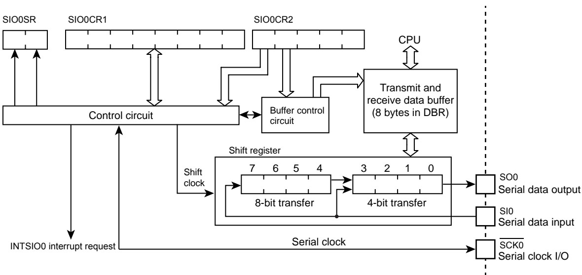
Figure 12-1 Serial Interface
