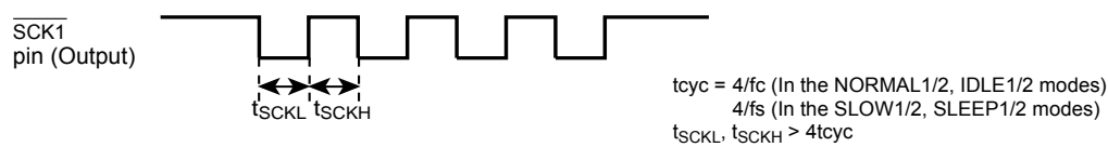
Figure 13-4 External clock pulse width
