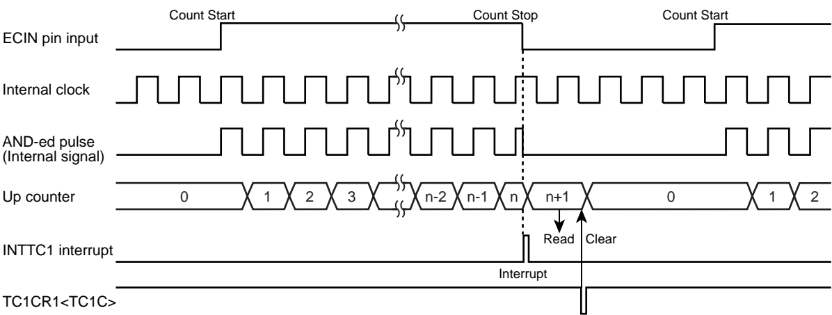
Figure 8-3 Pulse width measurement mode timing chart
