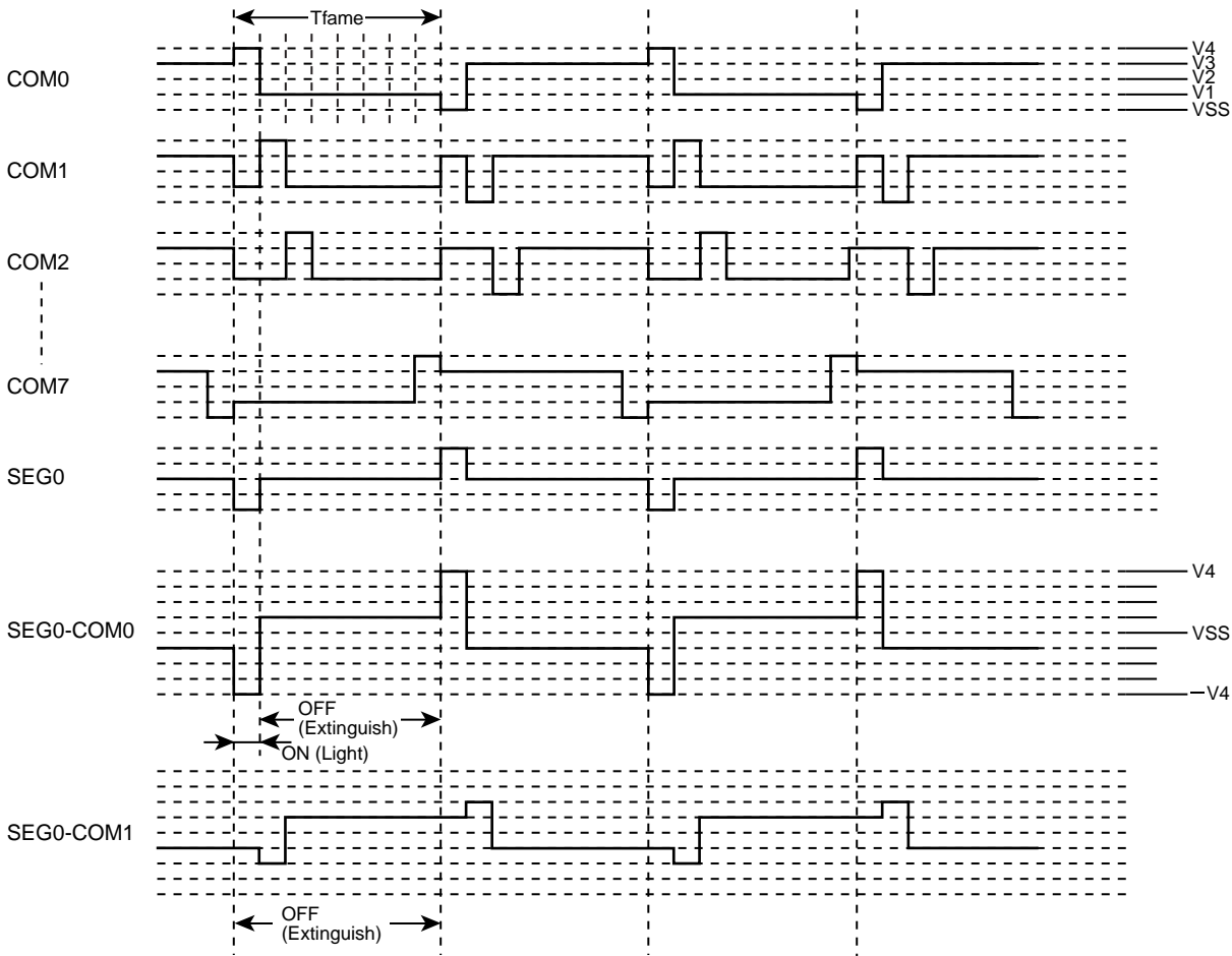
Figure 16-5 Example of Display Timing (1/8 duty)
