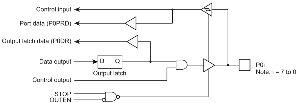
Figure 5-2 Port P0
