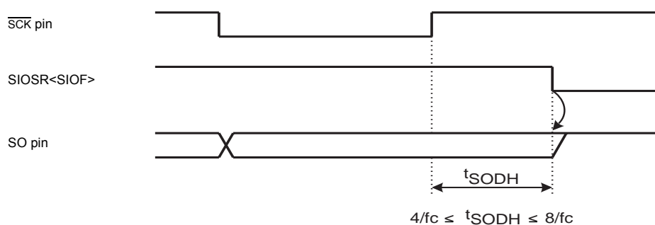
Figure 11-8 Hold Time of the End of Transmit Mode
