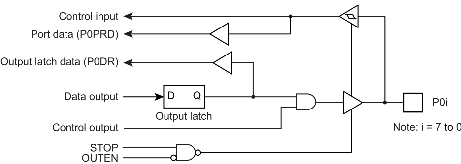
Figure 7-2 Port P0
