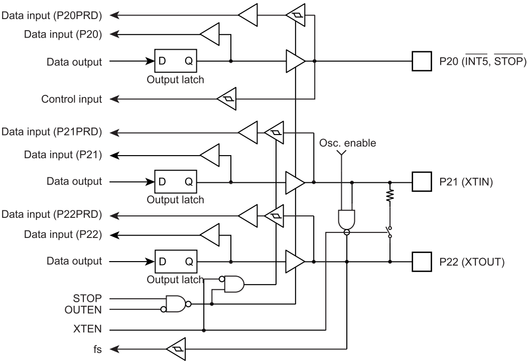
Figure 7-4 Port P2
