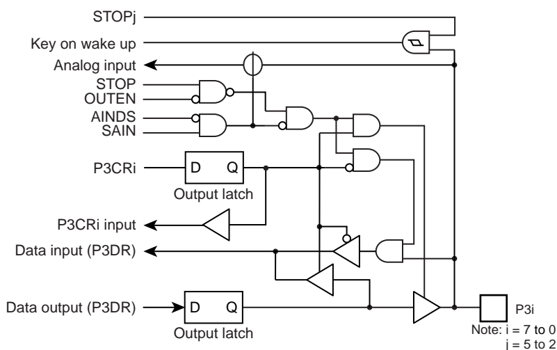
Figure 7-5 Port P3
