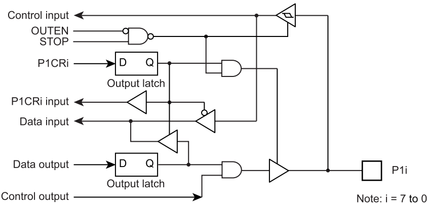
Figure 7-3 Port P1
