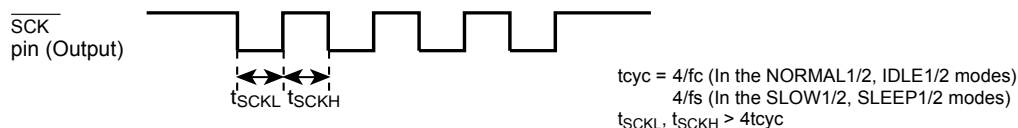
Figure 11-4 External clock pulse width
