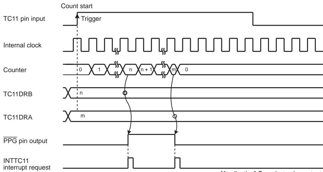
[Application] One-shot pulse output
