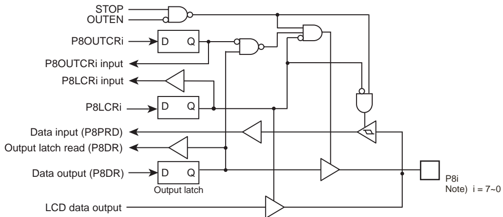
Figure 5-10 Port P8
