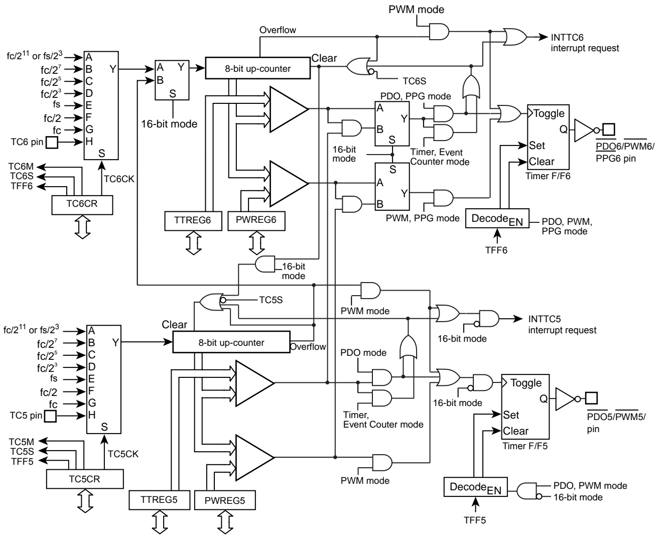
Figure 10-1 8-Bit TimerCounter 5, 6
