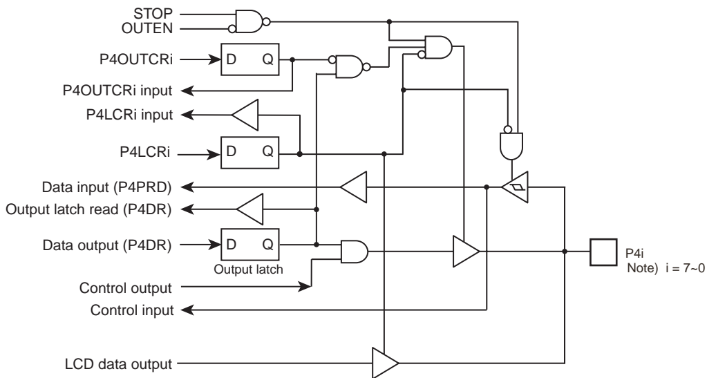
Figure 5-6 Port P4
