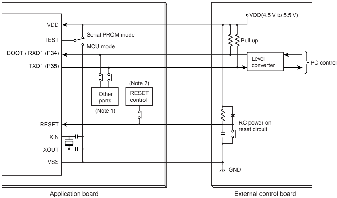
Figure 18-3 Example Connection for On-Board Writing
