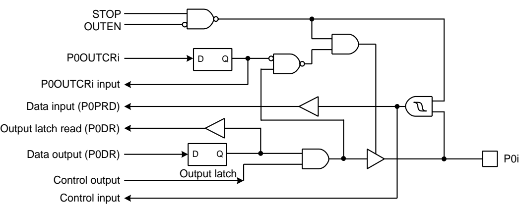
Figure 5-2 Port 0 and P0OUTCR
