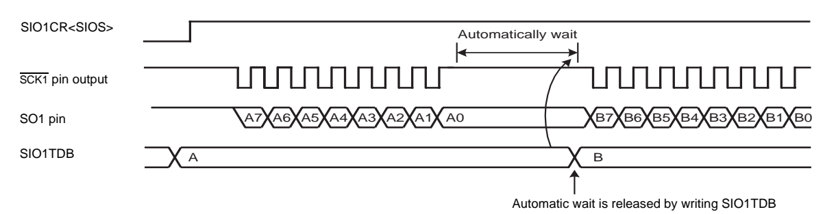
Figure 14-2 Automatic-wait Function (Example of transmit mode)
