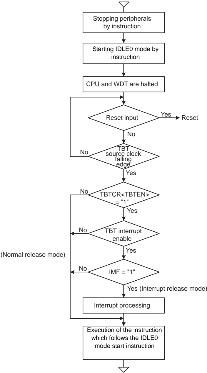
Figure 2-12 IDLE0 Mode
