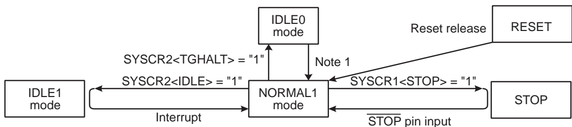
Figure 2-6 Operating Mode Transition Diagram
